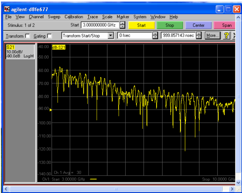
Fig. 3. Channel Transfer Function Measured with the Agilent E8363B Network Analyzer
