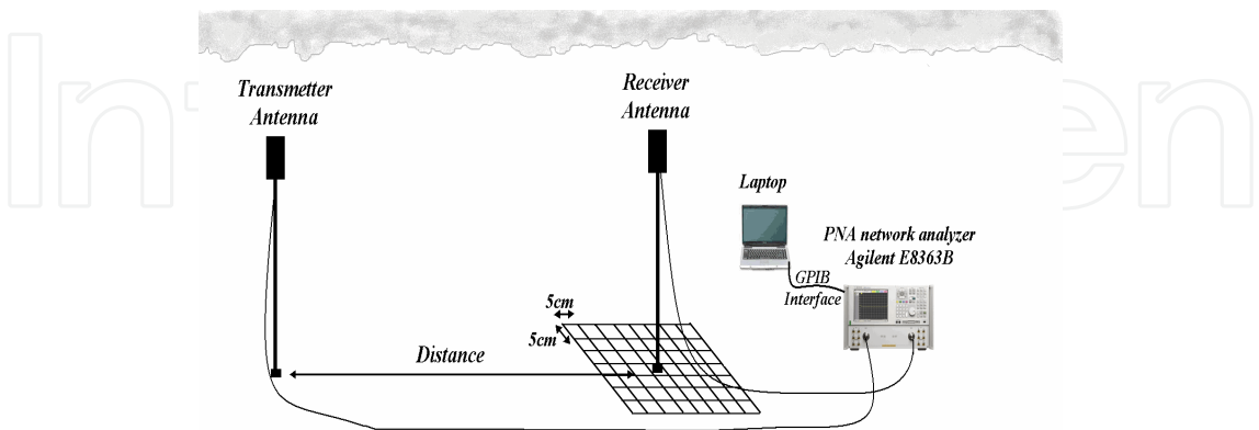
Fig. 2. Overview of the Measurement Setup
