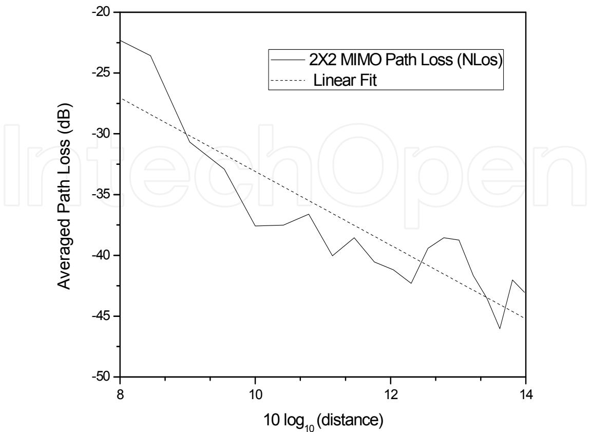
Fig. 17. Average Path versus distance in NLOS scenario
