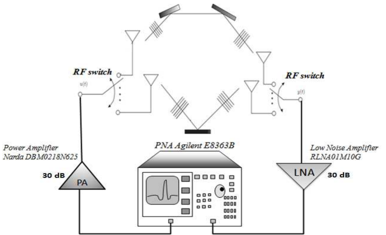
Fig. 13. Measurement setup
