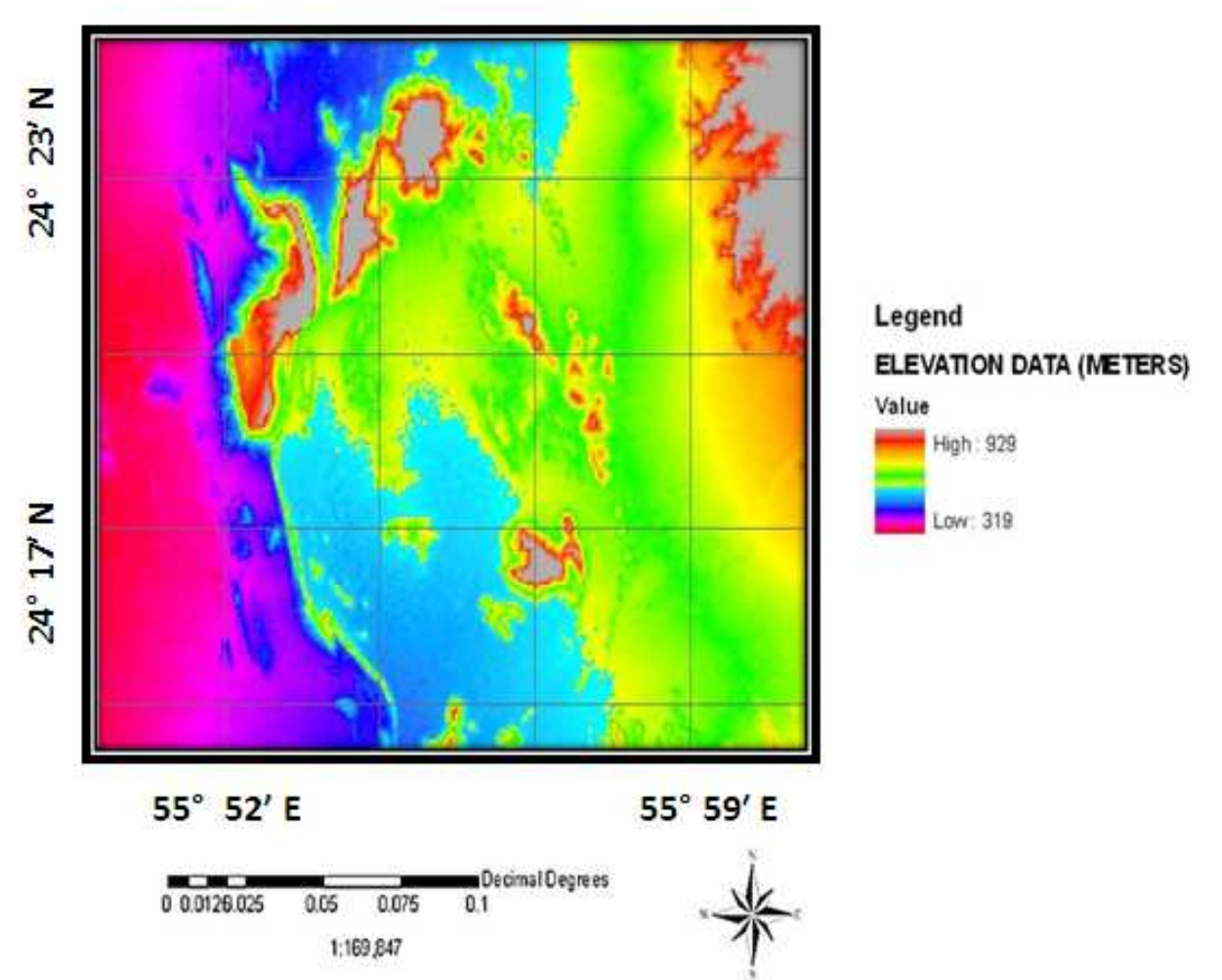
Fig. 7. DEM for study area.
