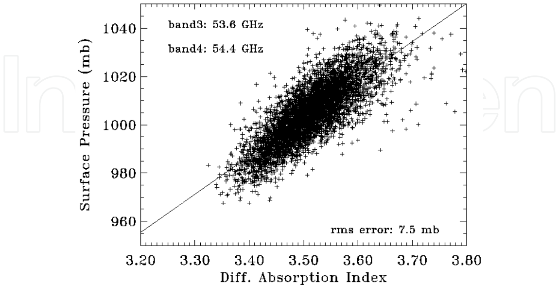
Fig. 9. Simulated relationship between the differential absorption index, the logarithm of the radar spectrum ratio at wavelengths 53.6 and 54.4 GHz , and surface air pressure.
