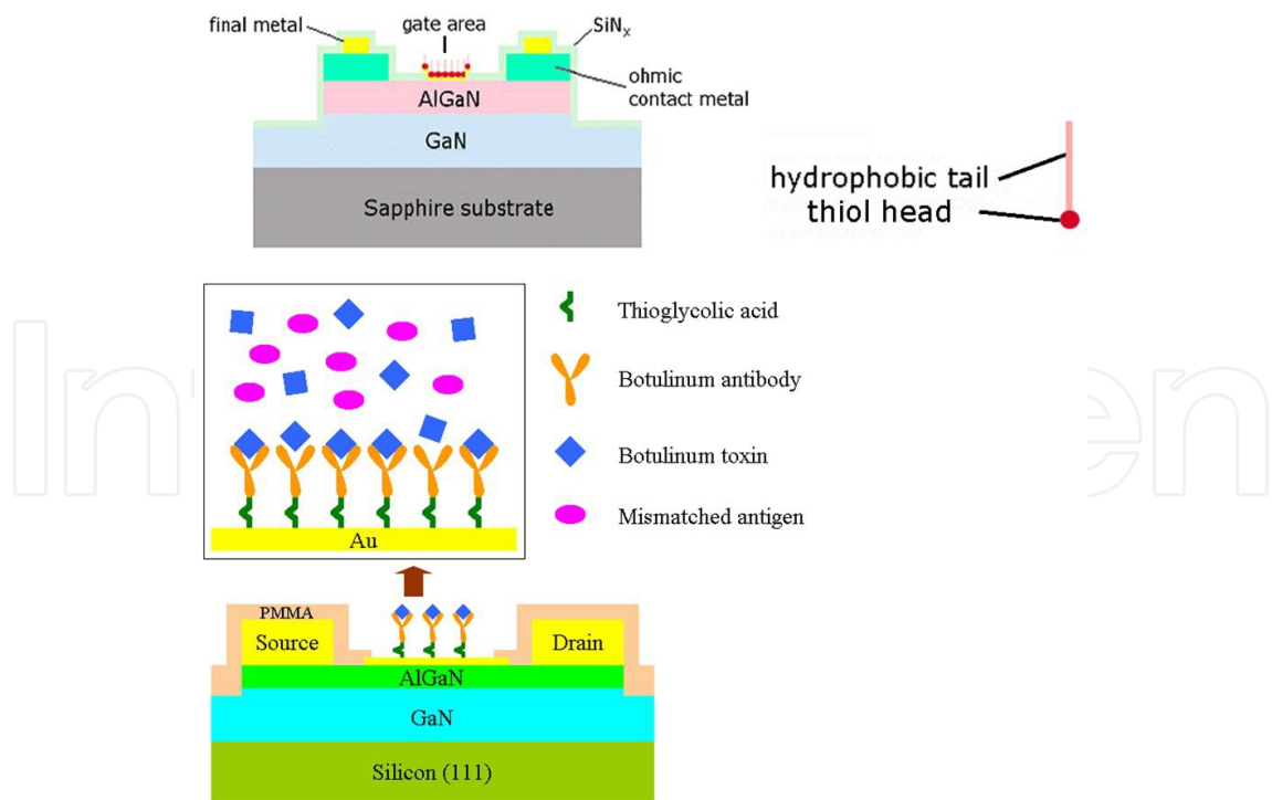
Figure 4. Schematic of AlGa N /Ga N HEMT. The Au-coated gate area was functionalized with thioglycolic acid for botulinum detection.
