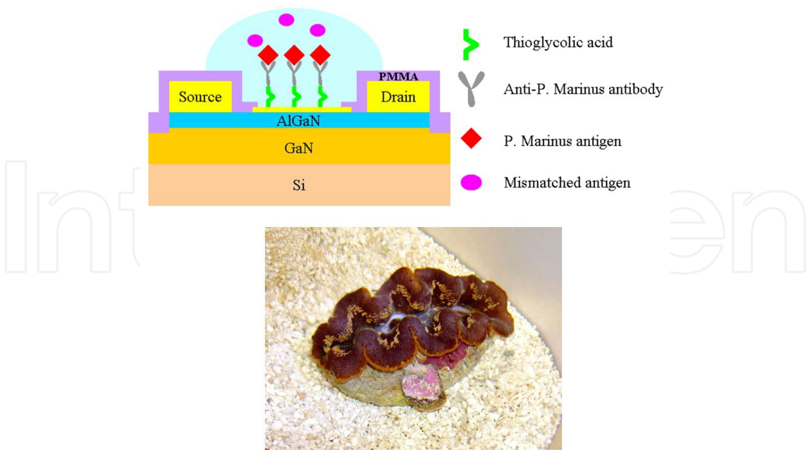
Figure 18. (top) Schematic of AlGaIn/GaN HEMT sensor. The gate area was functionalized with anti-P. marinus antibody on thioglycolic acid. (bottom) A picture of the clam, which may carry the perkinsus.
