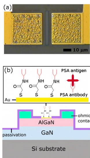
Figure 9. Schematic of HEMT sensor functionalized for PSA detection.
