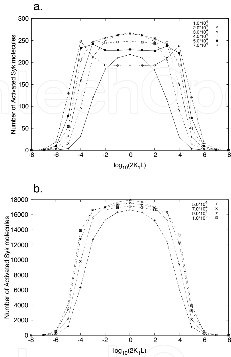
Fig. 2. Syk Activation curves for k_{+1} = 2.5 \times 10^6 \text{ M}^{-1}\text{s}^{-1} , k_{+2} = 8 \times 10^{-9} \text{ cm}^2\text{s}^{-1} , k_{-1} = k_{-2} = 0.01 \text{ s}^{-1} , and [Lyn]_{tot} = 10^5 per cell. Each curve corresponds to a different number of receptors per cell given in the legend. The number of activated Syk molecules on the y axis are given in numbers per cell. (a) [Syk]_{tot} = 5 \times 10^3 per cell; (b) [Syk]_{tot} = 6 \times 10^4 per cell. The number of activated Syk molecules on the y axis are the numbers per cell. In (a) the ratio of total receptors to total Syk varies from 2-14 while in (b) the same ratio varies from 0.83-1.67.
