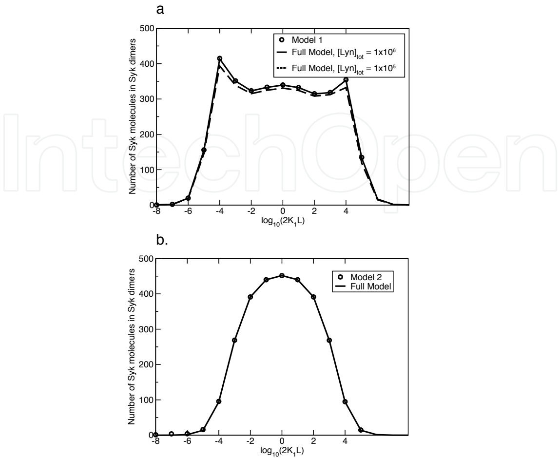
Fig. 6. Comparison of number of Syk dimers per cell obtained using reduced model 1 and 2, with the corresponding numbers obtained using the full model. [Syk]_{tot} = 7 \times 10^3 per cell; [FceRI]_{tot} = 10^5 per cell. We use the same ligand-receptor and Syk- p\gamma binding and unbinding parameters as in Table 2 for both the reduced models and the full model. (a) We consider two different total cellular concentrations of Lyn in the full model, [Lyn]_{tot} = 10^5 and [Lyn]_{tot} = 10^6 per cell. (b) Comparison of reduced model 2 to the full model when Lyn is in large excess and the rate of dephosphorylation is negligible ( [Lyn]_{tot} = 10^8 per cell, k_{-p} = 10^{-4}s^{-1} ).
