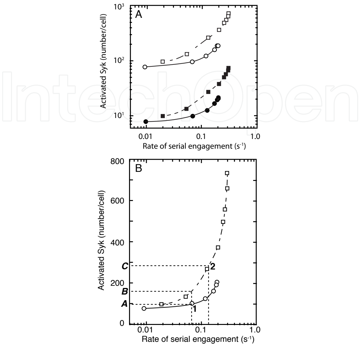
Fig. 13. Predicted number of activated Syk (Syk transphosphorylated by Syk) as a function of the rate of serial engagement. (A) The circles refer to bivalent ligand simulations and the squares to trivalent ligand simulations. Open and solid symbols refer to 1000 and 100 receptors in aggregates respectively. (B) Replot of the bivalent and trivalent curves in (A) for 1000 receptors in aggregates. The symbol 1 corresponds to a dimer with k_{+2}R = 0.01 s^{-1} and k_{off} = 0.10 s^{-1} . The symbol 2 corresponds to a trimer with the same rate constants. A = 100 , B = 161 and C = 290 activated Syk per cell. The net increase in activated Syk, (C - A) is 190 Syk per cell, of which C - B = 129 Syk per cell can be attributed to serial engagement.
