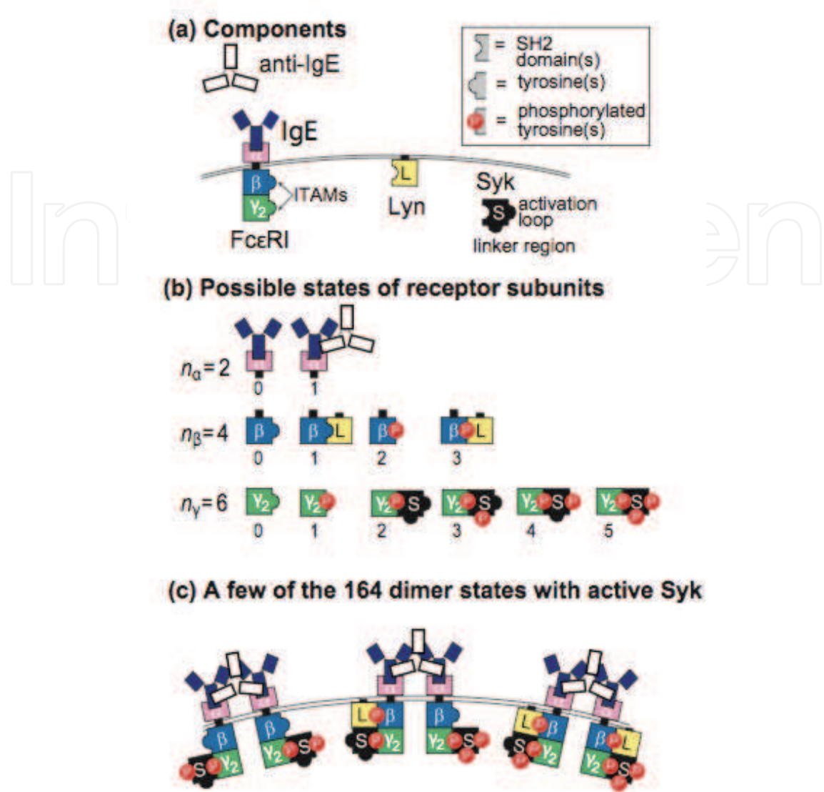
Fig. 1. Components and states of the model, modified from Faeder et al. (2003). The bivalent ligand is a monoclonal anti-IgE that can dimerize receptors.
