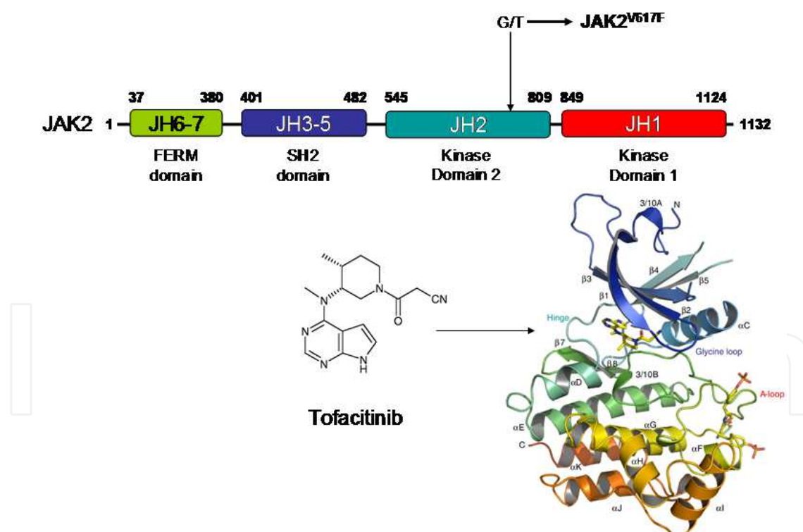
Fig. 1. Domain structure of human JAK2. The crystal structure of the JAK2 JH1 domain bound to JAK inhibitor tofacitinib is reproduced from Williams et al. (2009) with permission.
