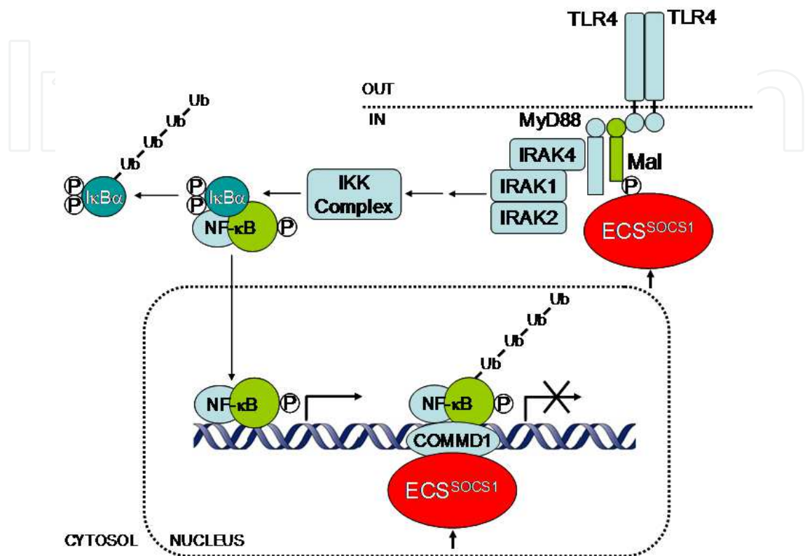
Fig. 4. Control of the NF- \kappa B pathway at multiple levels by a elongin-cullin-SOCS1 (ECS SOCS1 ) ubiquitin E3 ligase complex.
