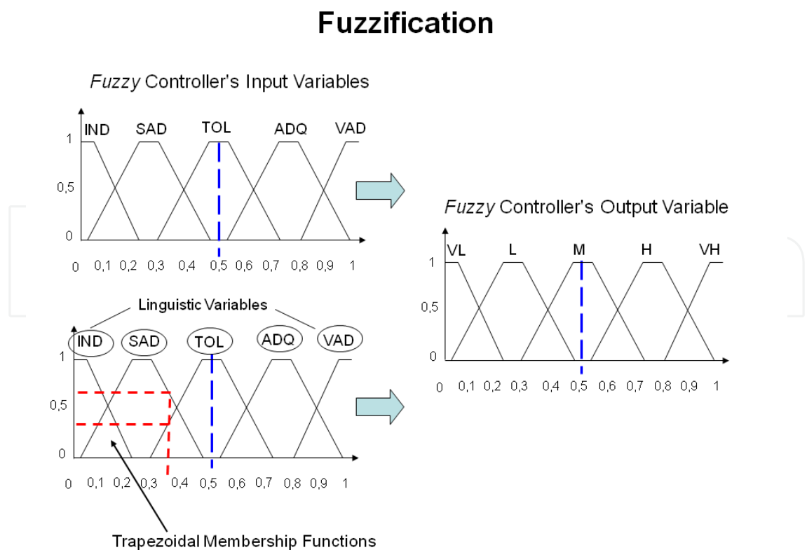
Fig. 2. Input controller's input and output membership functions
