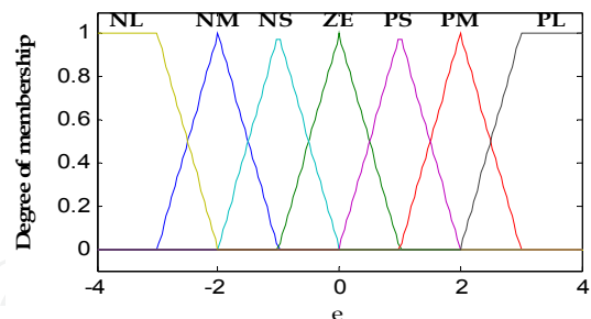
Fig. 5. The Membership function of input e(k).
