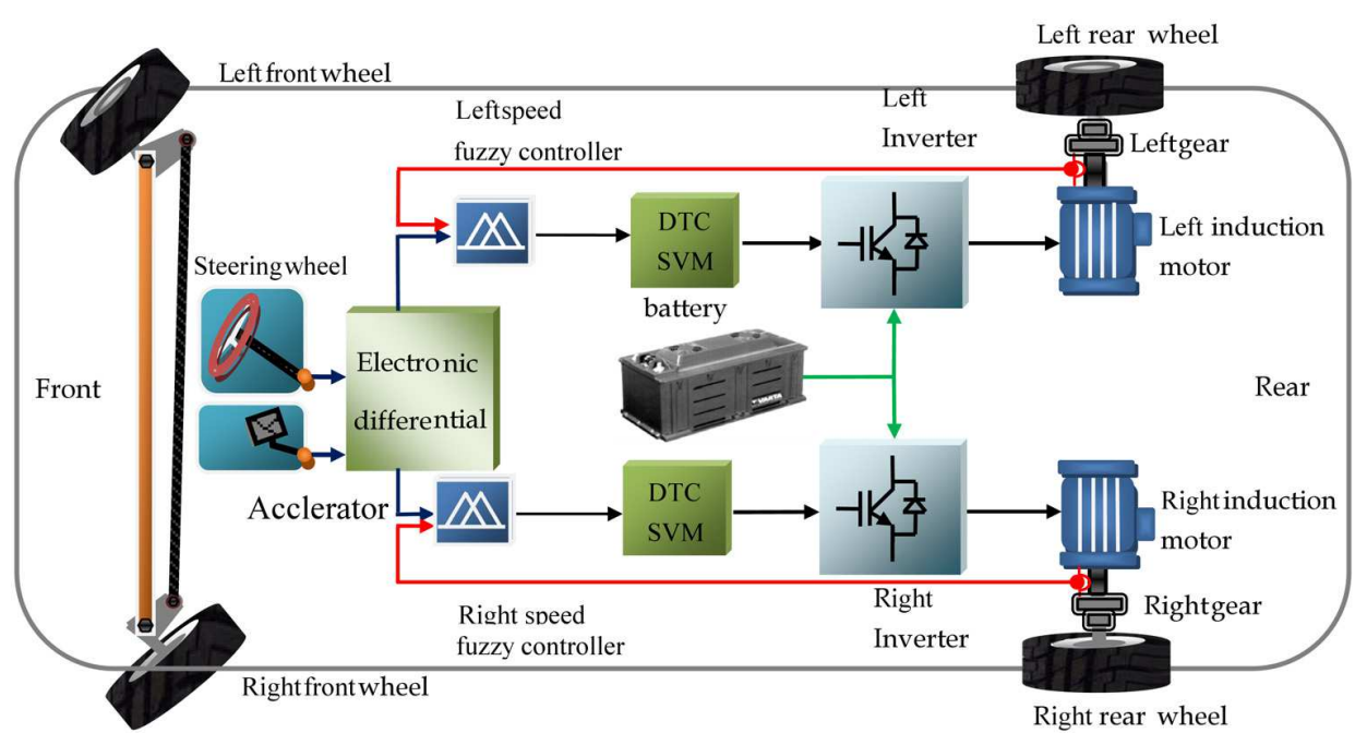
Fig. 13. The driving wheels control system
