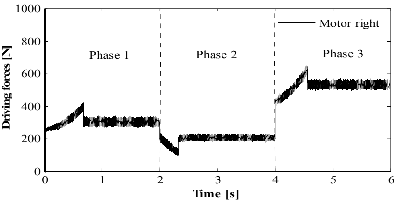
Fig. 18. Variation of driving force of the right motor in different phases.
