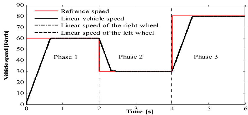
Fig. 15. Variation of vehicle speeds in different phases.
