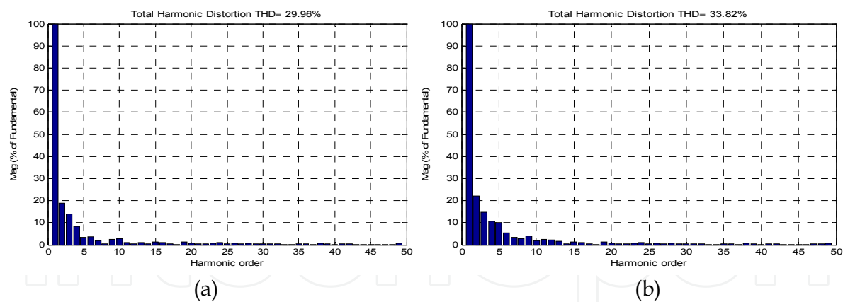
Fig. 22. (a) Total harmonic distortion using DTC with intelligent fuzzy PI controller, (b) Total harmonic distortion using DTC-SVM with classical PI.
