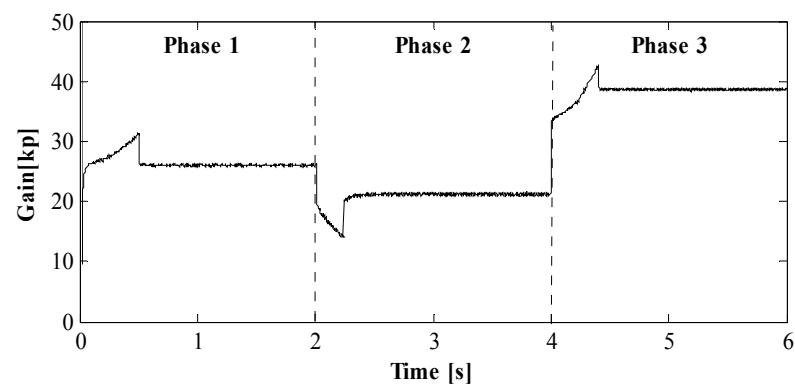
Fig. 20. Variation gain kp of intelligent fuzzy PI controller
