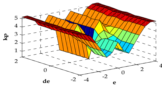
Fig. 9. View plot surface of fuzzy controller for k_p
