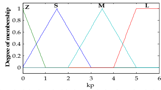
Fig. 7. The Membership functions of output k_p .
