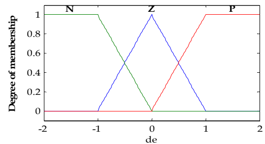
Fig. 6. The Membership function of input Δe(k) .
