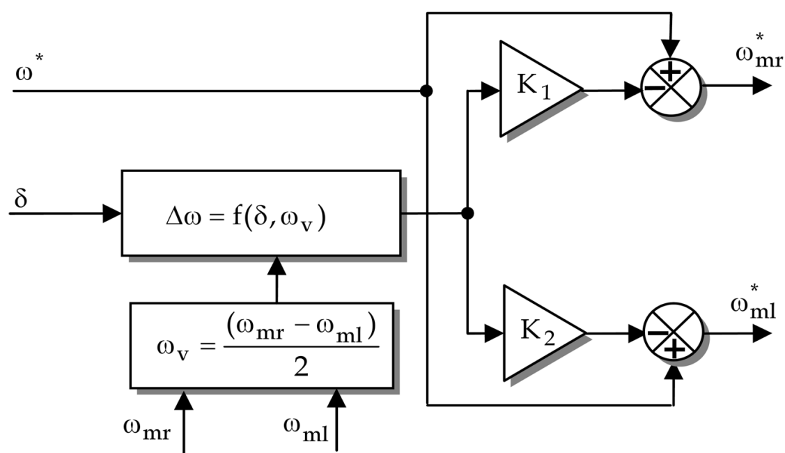
Fig. 11. Differential electronic.
