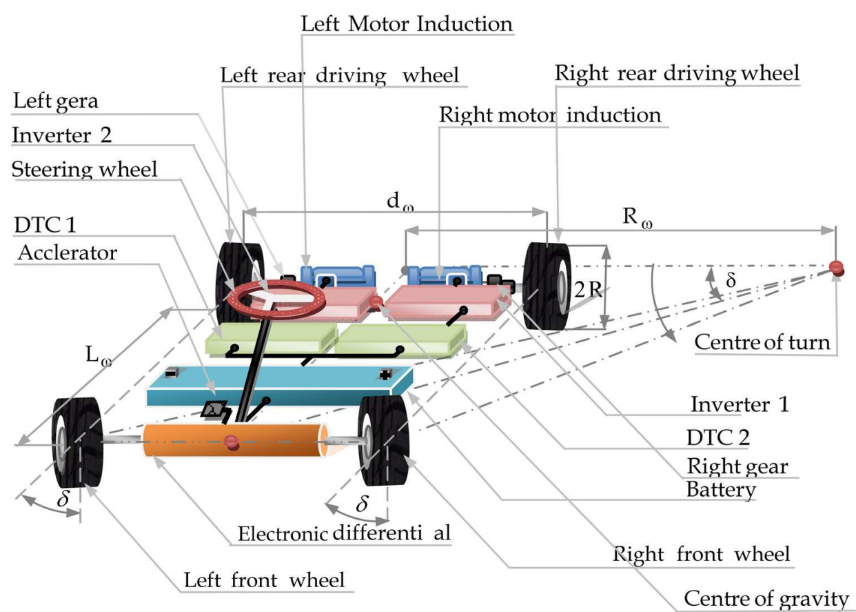
Fig. 12. Structure of vehicle in curve
