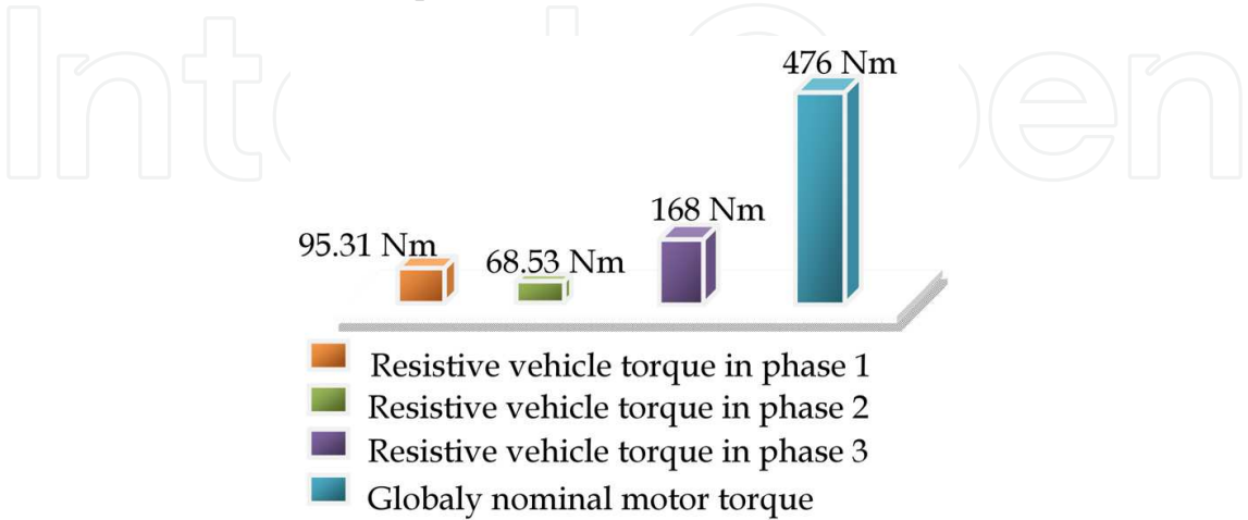
Fig. 19. Evaluation of the globally vehicle resistive torque compared to nominal motor torque in different phases.
