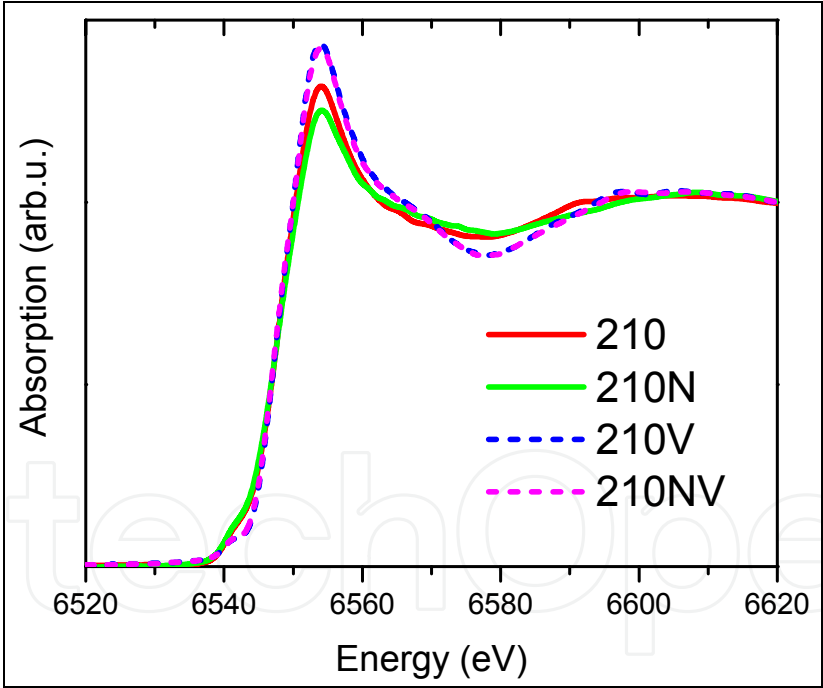
Fig. 19. XANES spectra of the as implanted and annealed samples.
