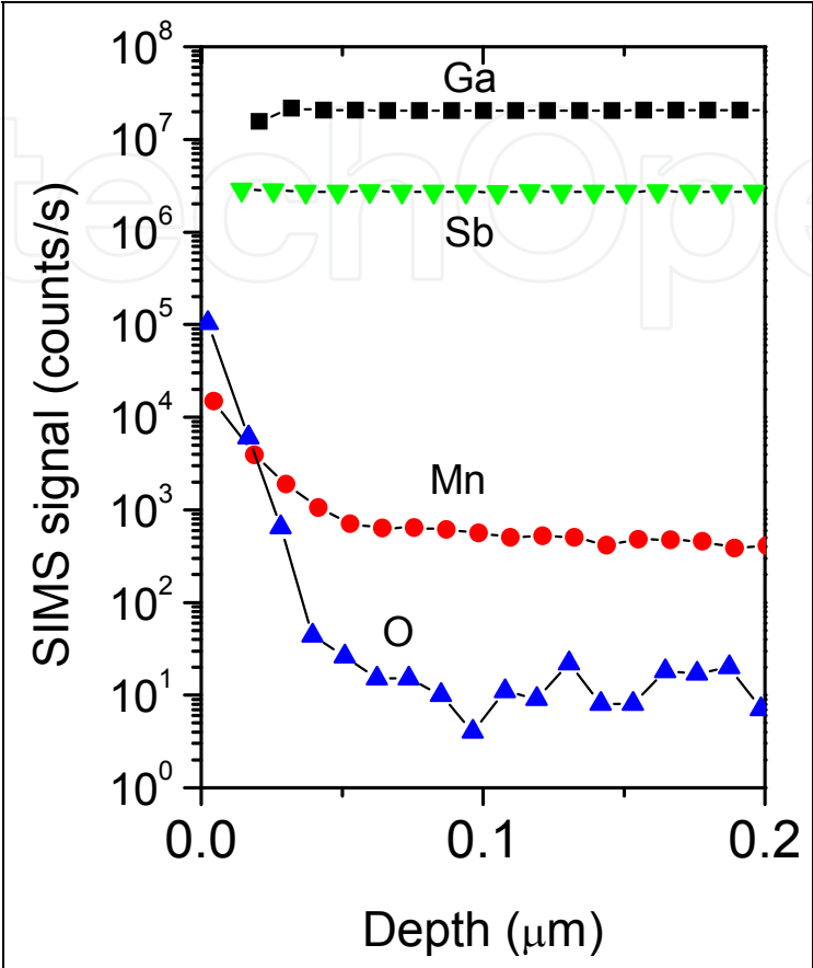
Fig. 3. SIMS depth profiles of the element distribution in the #2 sample.
