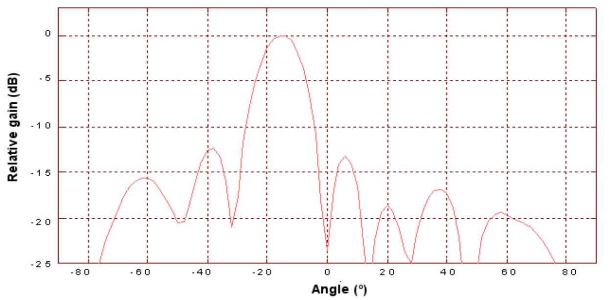
Fig. 5.8. Rx (-15)° beampattern with compensation for (-15)°
