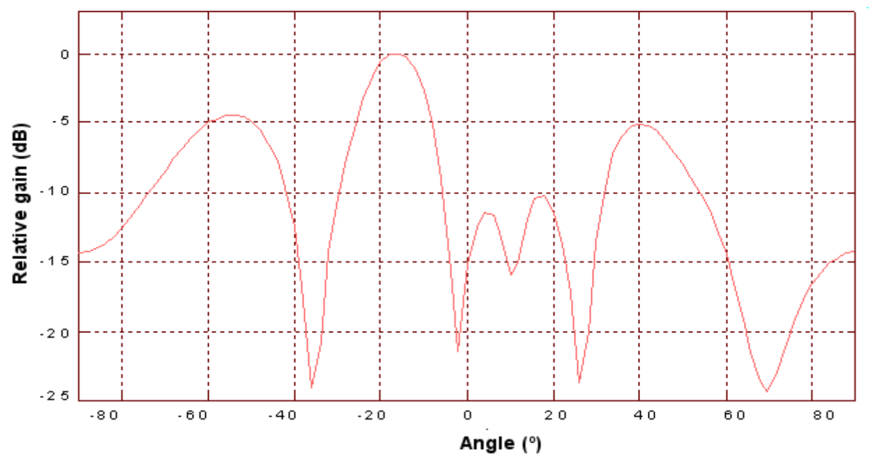
Fig. 5.7. Rx (-15°) beampattern with compensation for 0°
