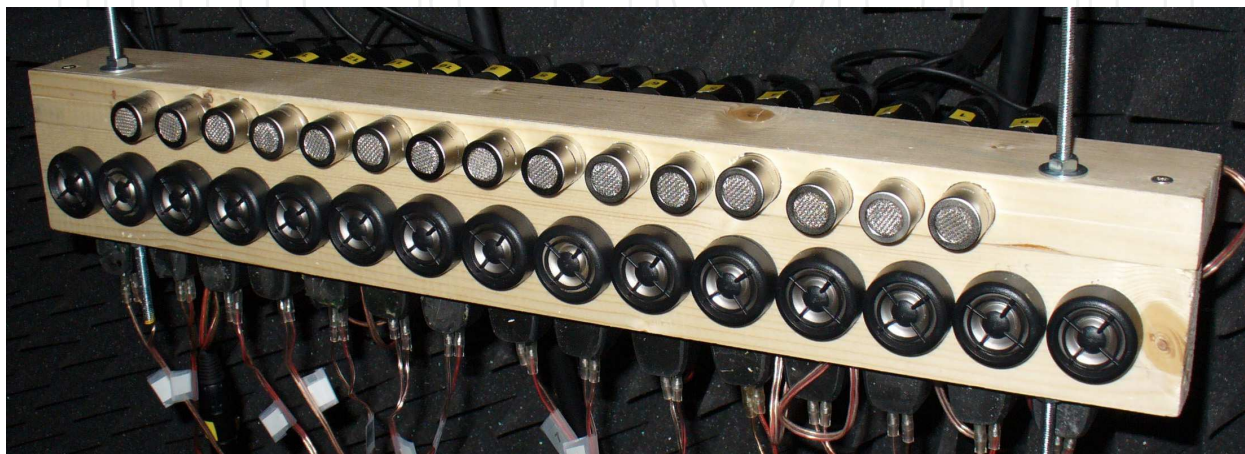
Fig. 2.1. Transmission (below) and reception (above) arrays
