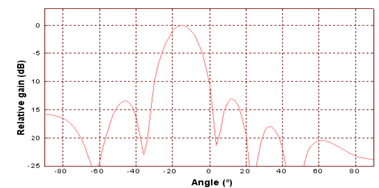
Fig. 5.4. Tx (-15)° beampattern with 0° compensation
