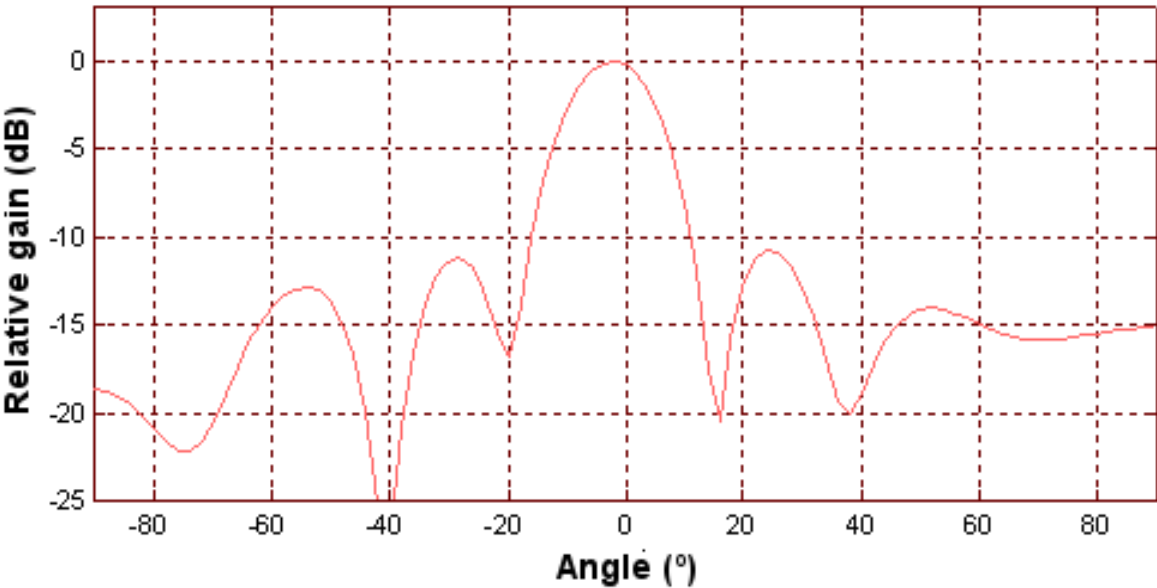
Fig. 5.2. Tx 0° beampattern without compensation
