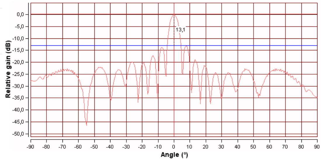
Fig. 3.5. Tx beampattern with compensation for 0°
