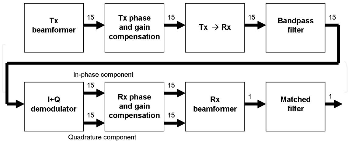
Fig. 2.2. Signal processing algorithm
