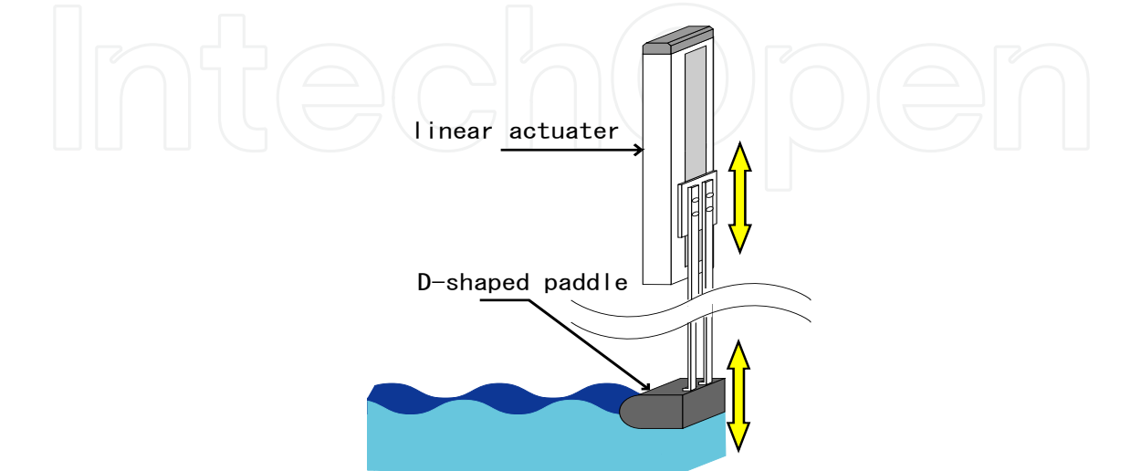
Fig. 2. A slide-type wavemaker with a D-shaped paddle
