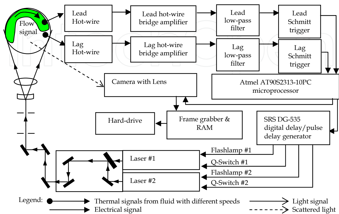
Fig. 4.a. Block diagram of the relationship between the triggers, laser and camera systems. The following establishes some criteria for the timing system of the microprocessor.
