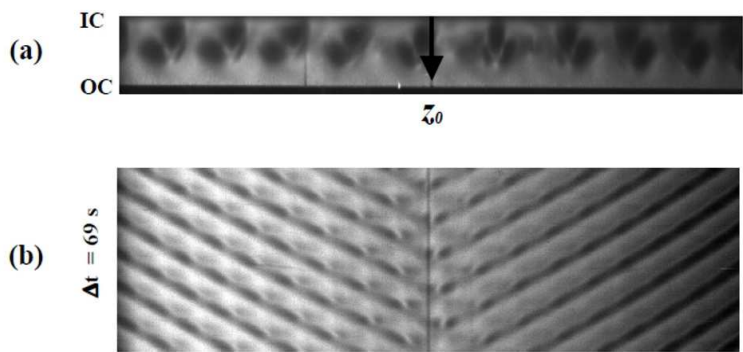
Fig. 5. Spiral pattern for Re_o = -230 and Re_i = 174 just above the critical value ( Re_{ic} = 160 , \epsilon = 0.0875 ): (a) cross-section of flow; (b) space- time diagrams I(z,t) taken in the mid-gap position ( x = 0.5 ) over the axial length \Delta z = 13.8 cm
