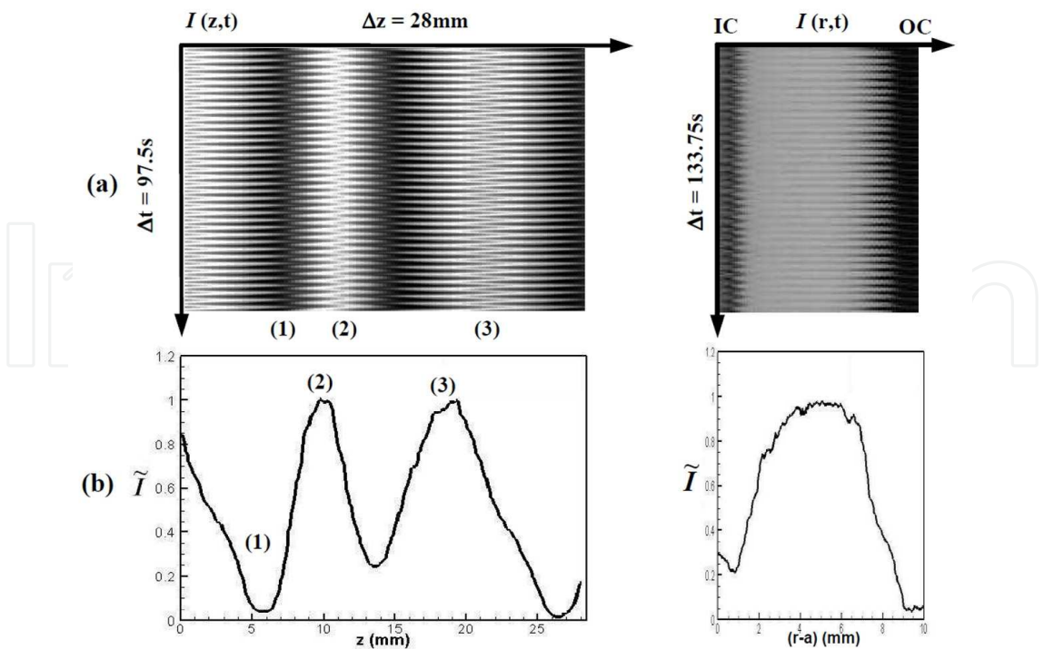
Fig. 17. a) Space-time diagrams of the intensity distribution in the axial I(z,t) and radial I(r,t) direction for Re_i = 880 . b) Radial profile and axial profile of light reflected intensity \tilde{I} = I / I_{\max} taken at \xi = 0.5 . (1) : vortex core, (2): inflow, (3): outflow.
