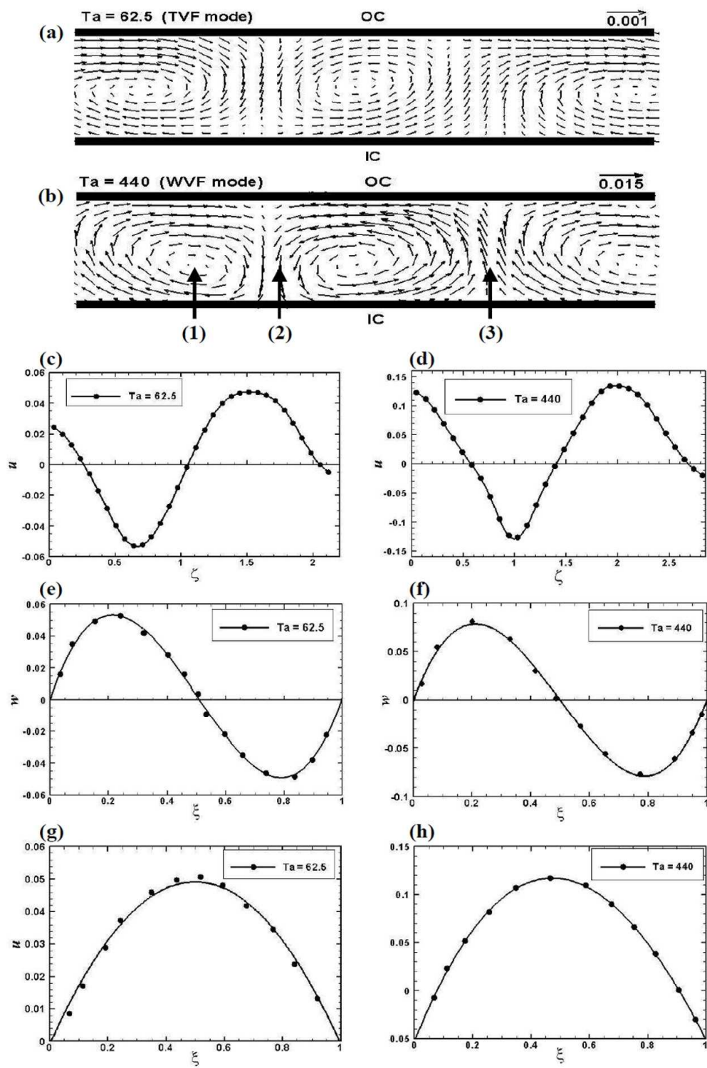
Fig. 10. a); b) Velocity field from PIV measurement; c-d) axial variation of velocity component u(\zeta) at the midgap ( \zeta = 0.5 ). Radial variation of velocity components: e-f) axial component w(\xi) in the vortex core (arrow (1)); and g-h) radial component u(\xi) at outflow (arrow (3)) for TVF ( Ta = 62.5 ), WVF ( Ta = 440 ) .
