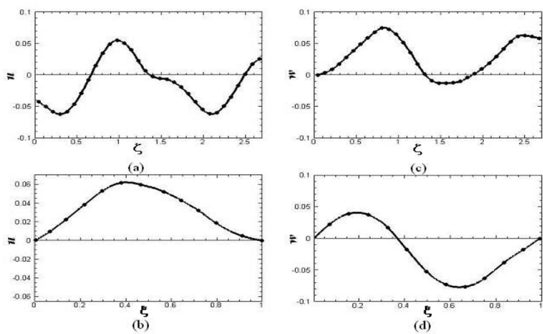
Fig. 23. Instantaneous velocity profiles u and w for Re_i = 212 , Re_o = -299 . Axial variation of velocity component at the midgap ( xi = 0.5 ) : a) u(zeta) and c) w(zeta) . Radial variation of velocity components: b) Radial component u(xi) at outflow, d) axial component w(xi) in the vortex core.
