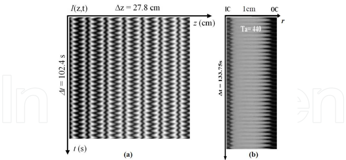
Fig. 4. Space-time diagrams for Wavy Vortex Flow ( Re_o = 0 ; Re_i = 880 ) cross section of which is shown in Fig. 2 : (a) axial distribution I(z,t) ; (b) radial distribution I(r,t) .
