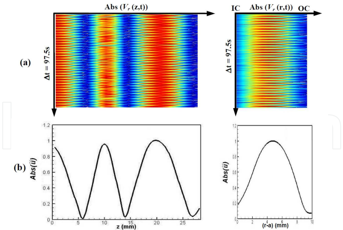
Fig. 18. a) Space-time diagrams of the absolute value of radial velocity component for Re_i = 880 , b) Radial and axial profiles of the absolute value \tilde{u} = V_r / V_{r\max} of the radial velocity component measured at \xi = 0.5 .
