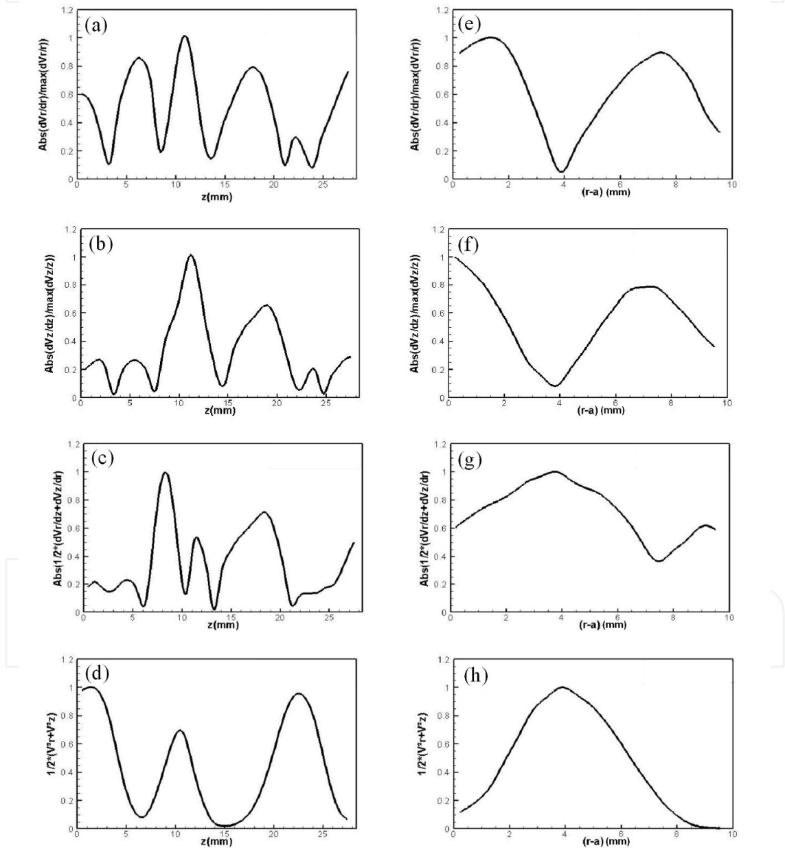
Fig. 19. Axial profiles of the absolute values of flow characteristics measured at \xi = 0.5 : a) \dot{\epsilon}_{rr} , b) \dot{\epsilon}_{zz} , c) \dot{\epsilon}_{rz} and d) kinetic energy E ; Radial profiles of the absolute values of flow characteristics measured in the outflow: e) \dot{\epsilon}_{rr} , f) \dot{\epsilon}_{zz} , g) \dot{\epsilon}_{rz} and h) kinetic energy E .
