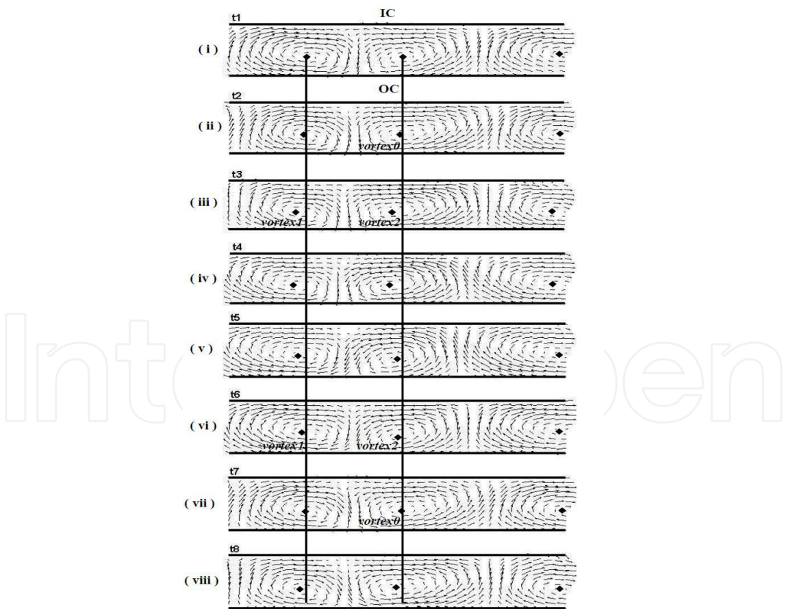
Fig. 13. The instantaneous velocity fields of WVF at Re_i = 880 for 8 records ( t_{i+1}=t_i+0.5s ), the time progresses from top to bottom through one complete cycle of an azimuthal wave passing the measurement plane
