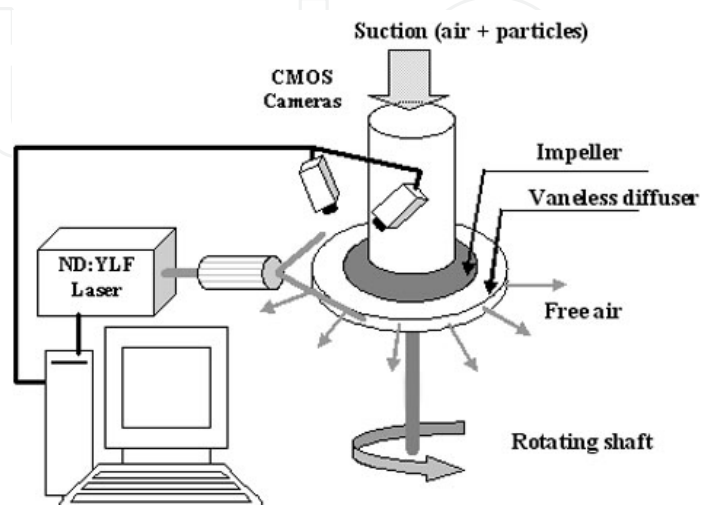
Fig. 12. Experimental set-up
