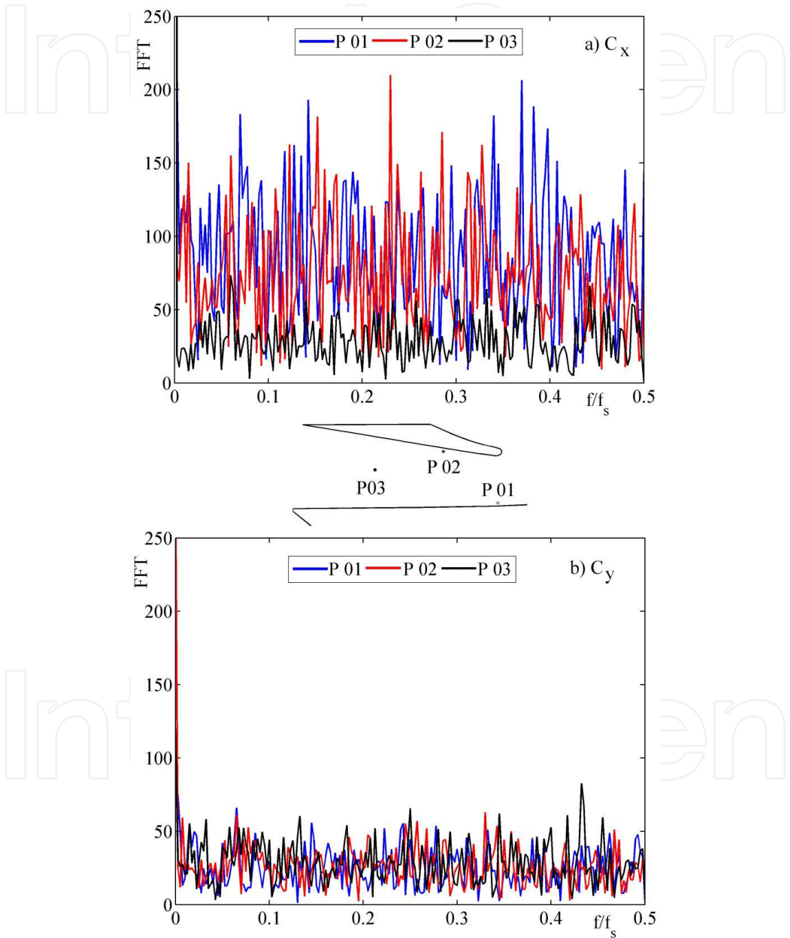
Fig. 8. FFT of the velocity components signals determined in three points of the diffuser passage: at the entrance near the suction side (blue line), near the blade pressure side (red line) and in the second half of the diffuser passage far from the blade profiles (black line). a) C_x b) C_y
