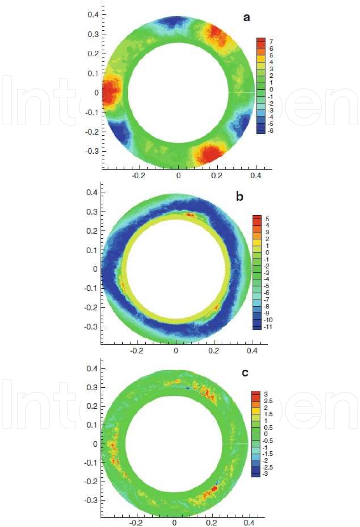
Fig. 16. Results of the averaging procedure: a) radial velocity; b) tangential velocity; c) axial velocity [m/s]
