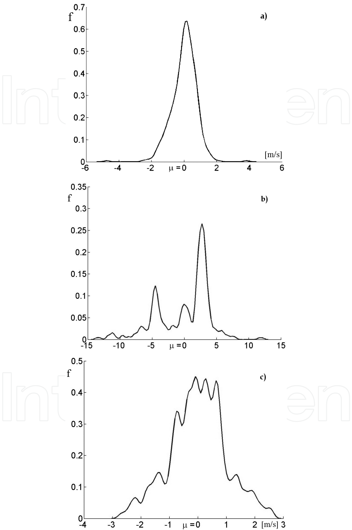
Fig. 5. Examples of probability density distributions of velocity values
