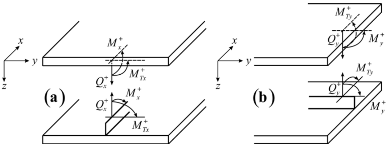
Fig. 2. Conventions for tensional forces, bending moments and torsional moments between upper panel and (a) x -wise and (b) y -wise stiffeners, which also hold at the interface between bottom panel and x - and y -wise stiffeners
