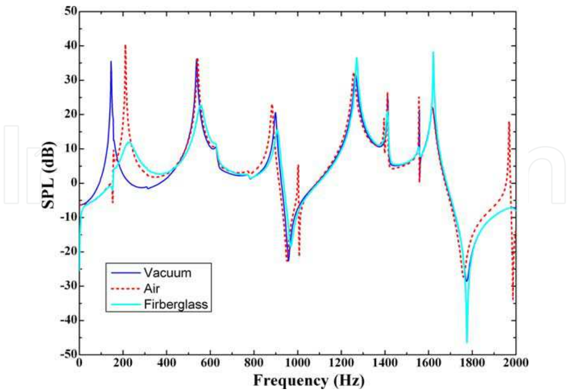
Fig. 7. Sound pressure levels radiated by different orthogonally rib-stiffened sandwich structures plotted as functions of frequency for stiffener separations ( l_x=0.35\text{m} , l_y=0.35\text{m} )
