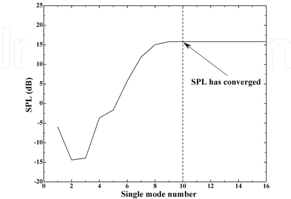
Fig. 3. Convergence check of numerical solution for sound radiation of an infinite orthogonally rib-stiffened sandwich structure with stiffener separations (l_x, l_y) = (0.20\text{m}, 0.20\text{m}) when excited by a harmonic point force at 10 kHz
