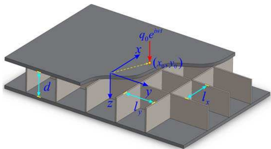
Fig. 1. Schematic illustration of orthogonally rib-stiffened sandwich structure (three different kinds: vacuum cavity, air cavity, and fiberglass filled cavity) excited by time-harmonic point force at (x_0, y_0)
