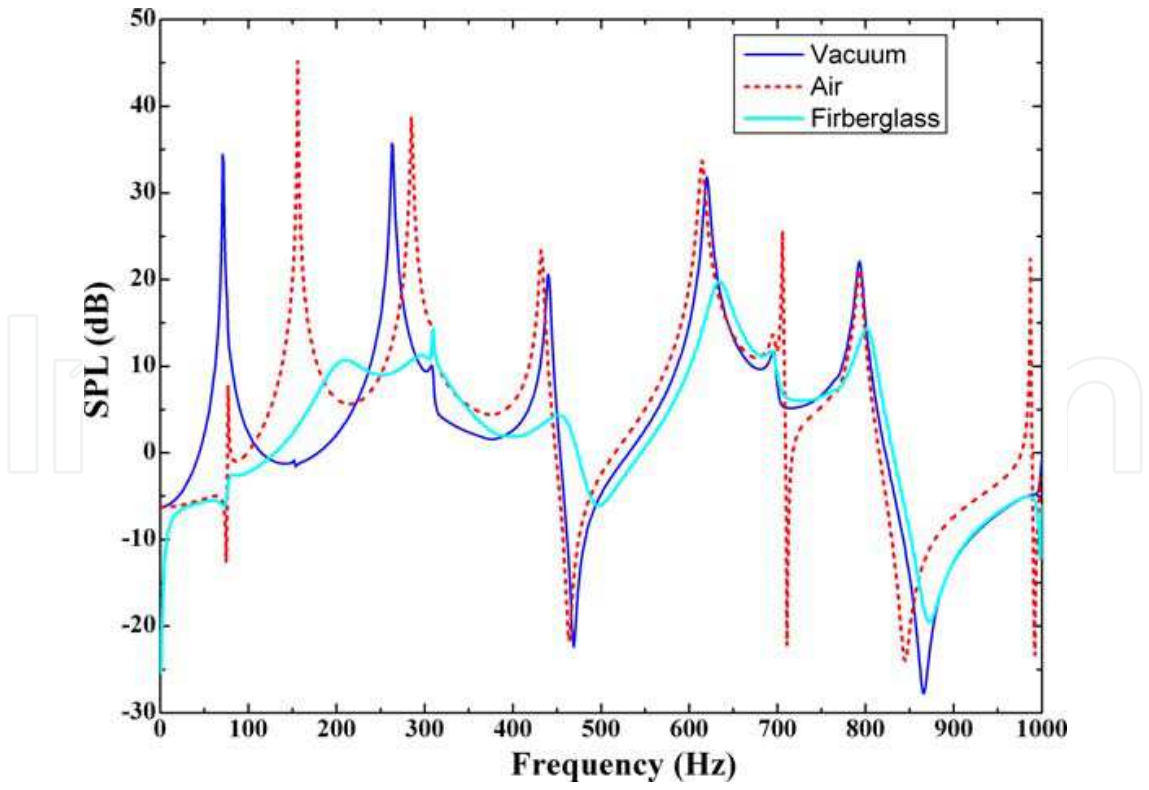
Fig. 8. Sound pressure levels radiated by different orthogonally rib-stiffened sandwich structures plotted as functions of frequency for stiffener separations ( l_x=0.50\text{m} , l_y=0.50\text{m} )
