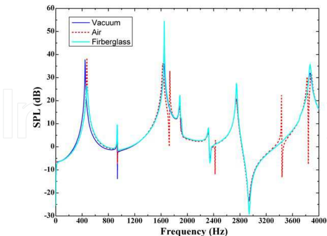
Fig. 6. Sound pressure levels radiated by different orthogonally rib-stiffened sandwich structures plotted as functions of frequency for stiffener separations (l_x, l_y) = (0.20\text{m}, 0.20\text{m})
