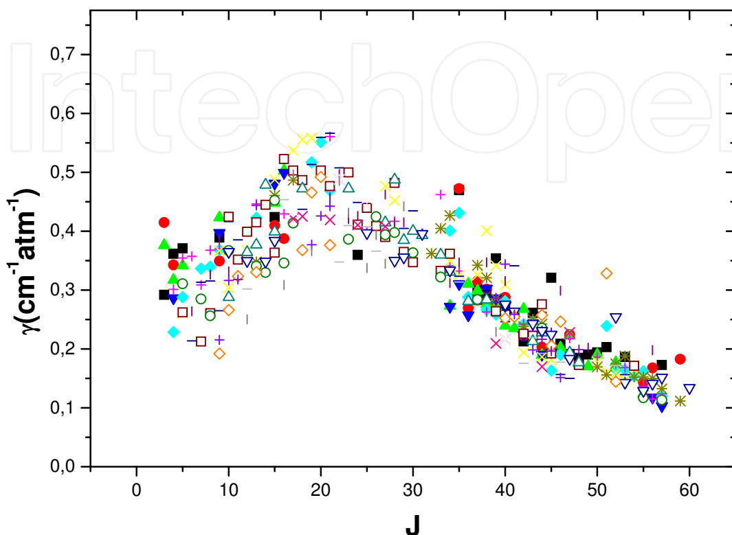
Fig. 11. Experimental self-broadening coefficients \gamma as function of the rotational quantum number J for the \nu_2 band PQ branch of ^{12}\text{CH}_3^{79}\text{Br} and ^{12}\text{CH}_3^{81}\text{Br} for K=0 to 9. For a given J value, the symbols indicate the different K -lines for which measurements are performed
