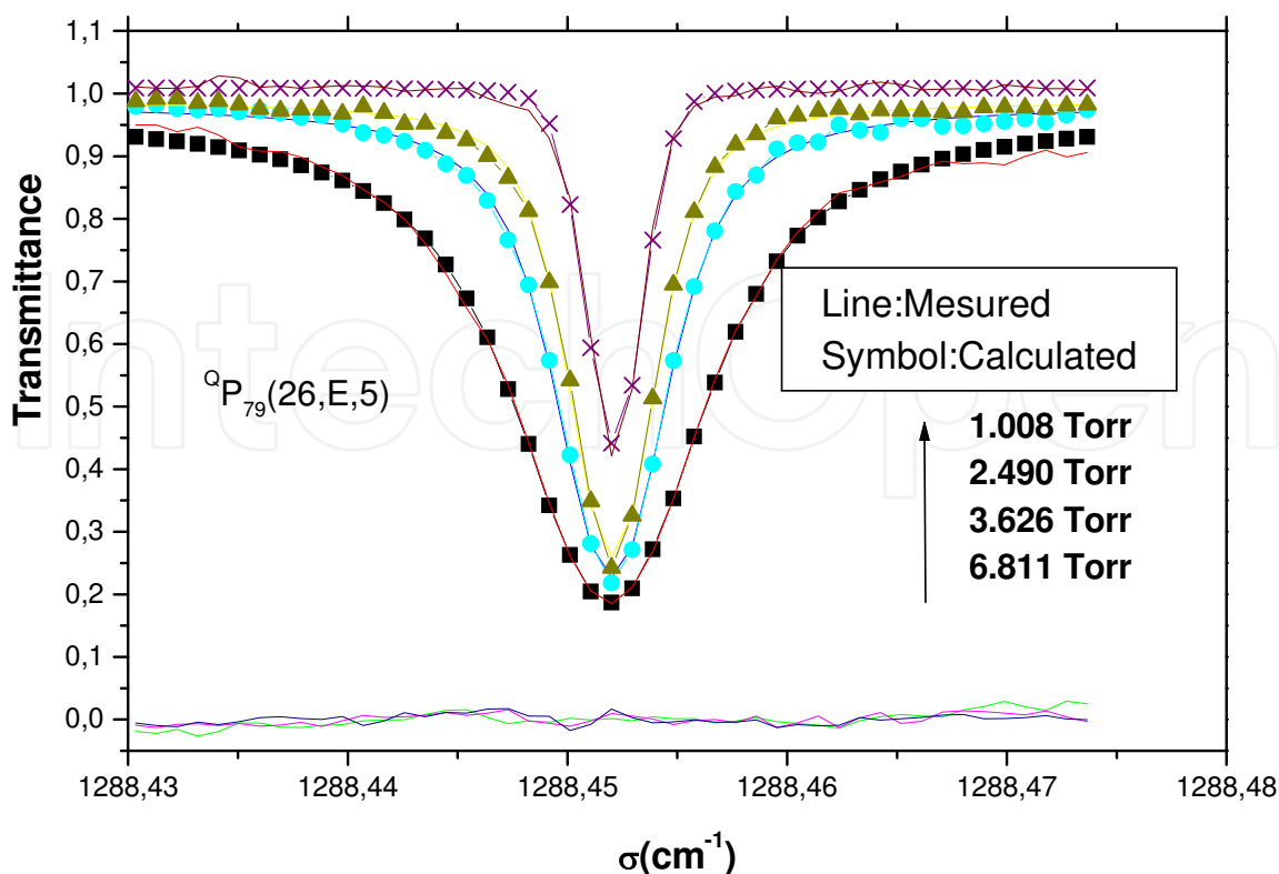
Fig. 7. Results of spectrum fits for the QP_{79}(26,E,5) line in the \nu_2 band of CH_3Br self-broadened at 296 K. (symbol) and (—) are, respectively, the calculated and measured values. Measured minus calculated deviations are shown in the lower part of the graph
