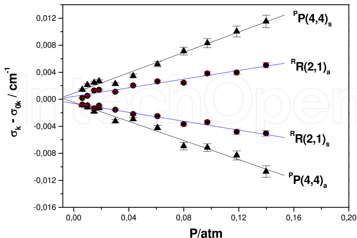
Fig. 13. Plots of the pressure-induced variation of \sigma - \sigma_0 versus \text{NH}_3 pressure P for the components of the doublets R_{as}R(2,1) and P_{as}P(4,4) of the \nu_4 band of \text{NH}_3 self-perturbed
