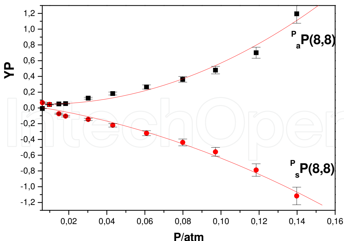
Fig. 14. Variation of PY as function of pressure P for the two components of ^{\text{P}}_{\text{as}}\text{P}(8,8) doublet of the \nu_4 band of \text{NH}_3 self-perturbed
