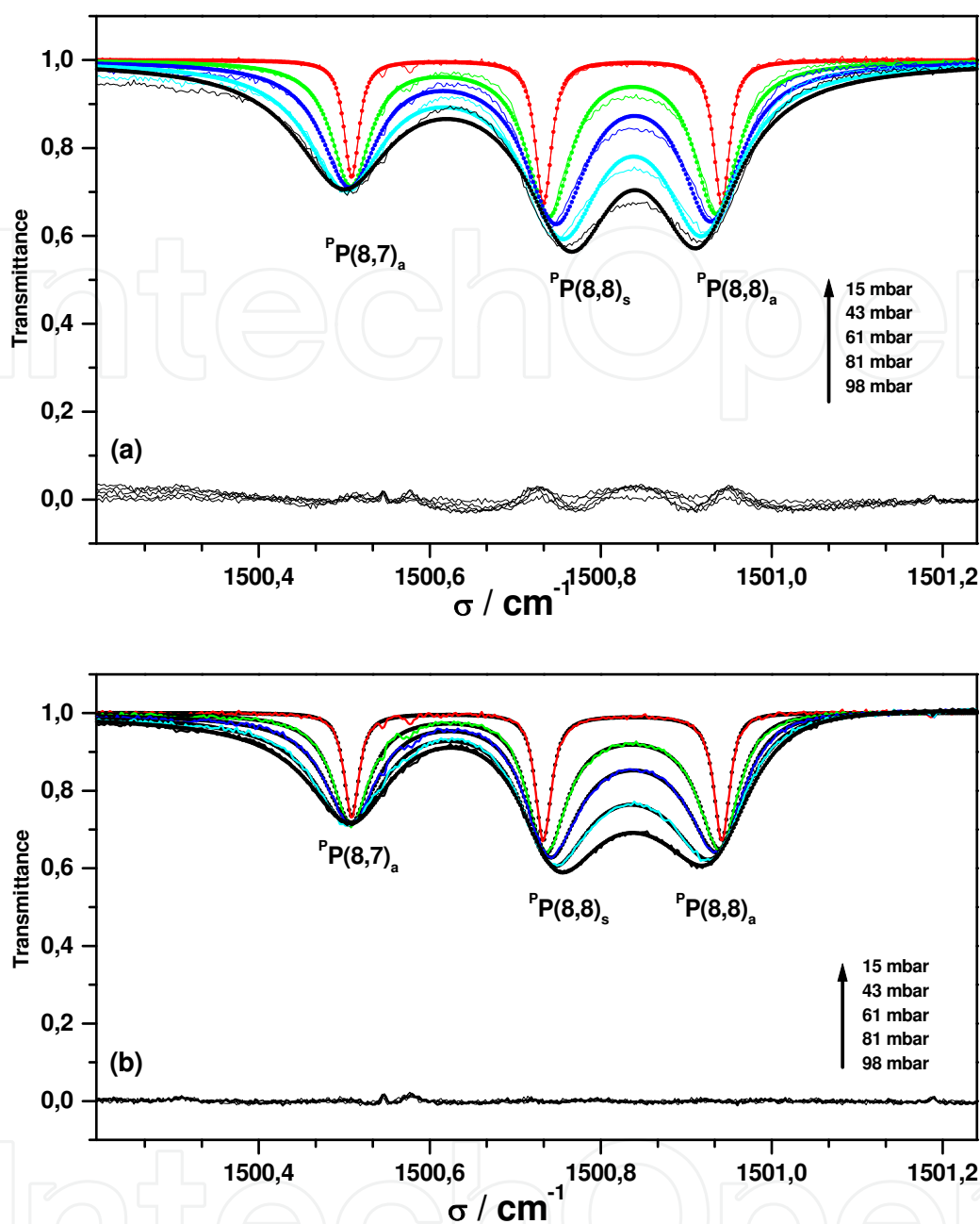
Fig. 6. Graphic demonstration of line-mixing obtained for pure \text{NH}_3 spectra for P_aP(8,7) line and P_{as}P(8,8) inversion doublet of the \nu_4 band at various pressures. (—) and (•) are the measured and calculated values, respectively. Measured minus calculated deviations are shown in the lower part of graphs. Plots (a) and (b) have been obtained without ( Y=0 ) and with ( Y \neq 0 ) the line-mixing, respectively. These plots illustrate the shift of P_{as}P(8,8) components line center towards each other
