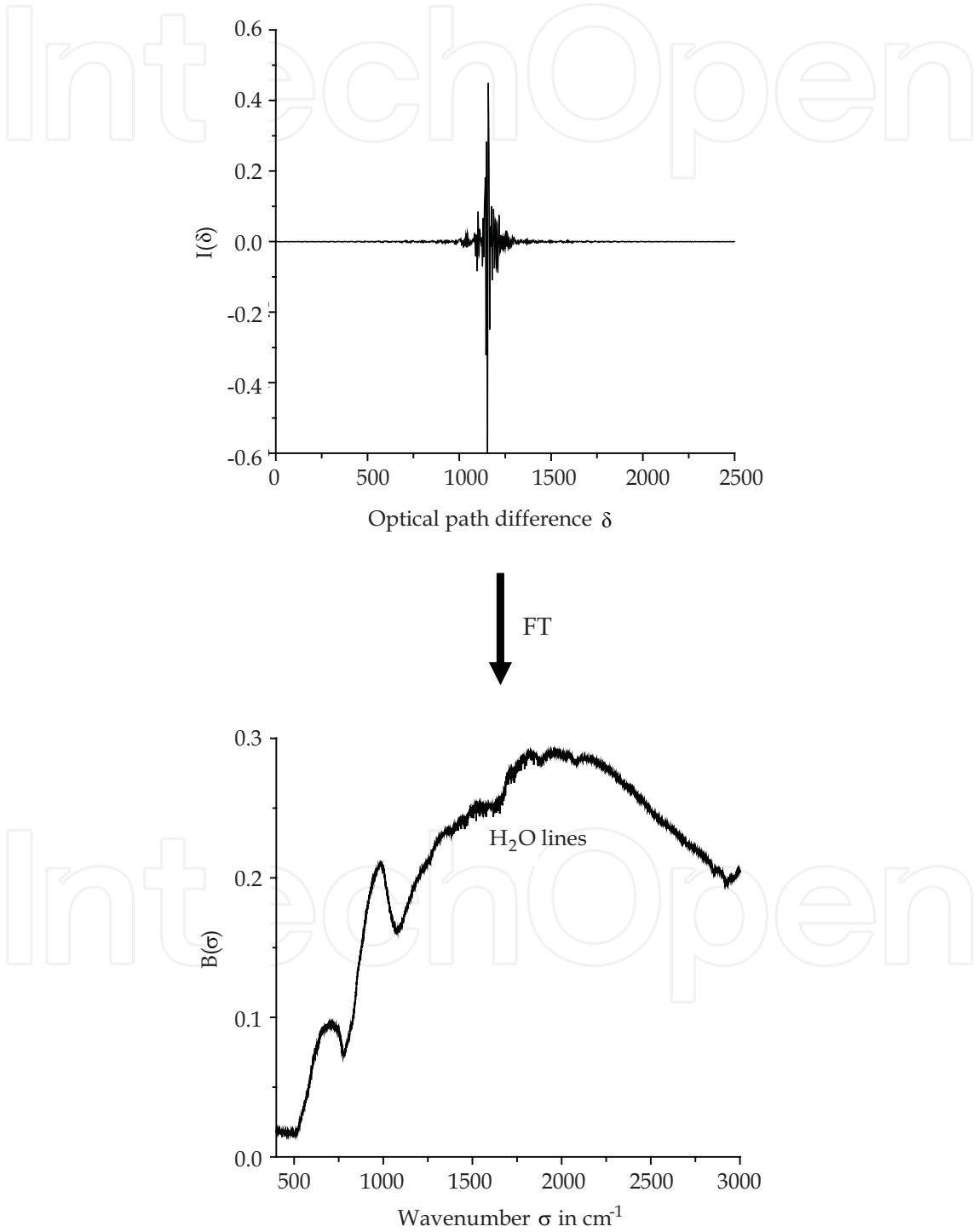
Fig. 2. Example of an interferogram and its spectrum calculated using a Fourier Transform algorithm
