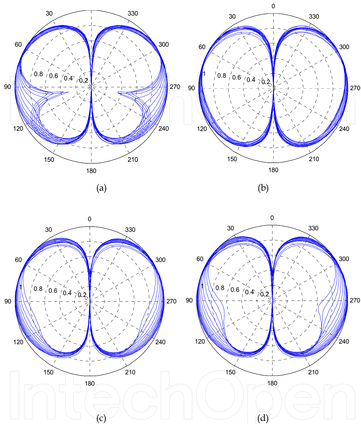
Fig. 3. Normalized Radiation Patterns v.s. frequency (a) conventional monopole, (b) PMC loaded monopole (case I), (c) PMC loaded monopole (case II) , and (d) PMC loaded monopole (case III). From (Jafargholi et al., 2010), copyright © 2010 by the Institute of Electrical and Electronics Engineers (IEEE).
