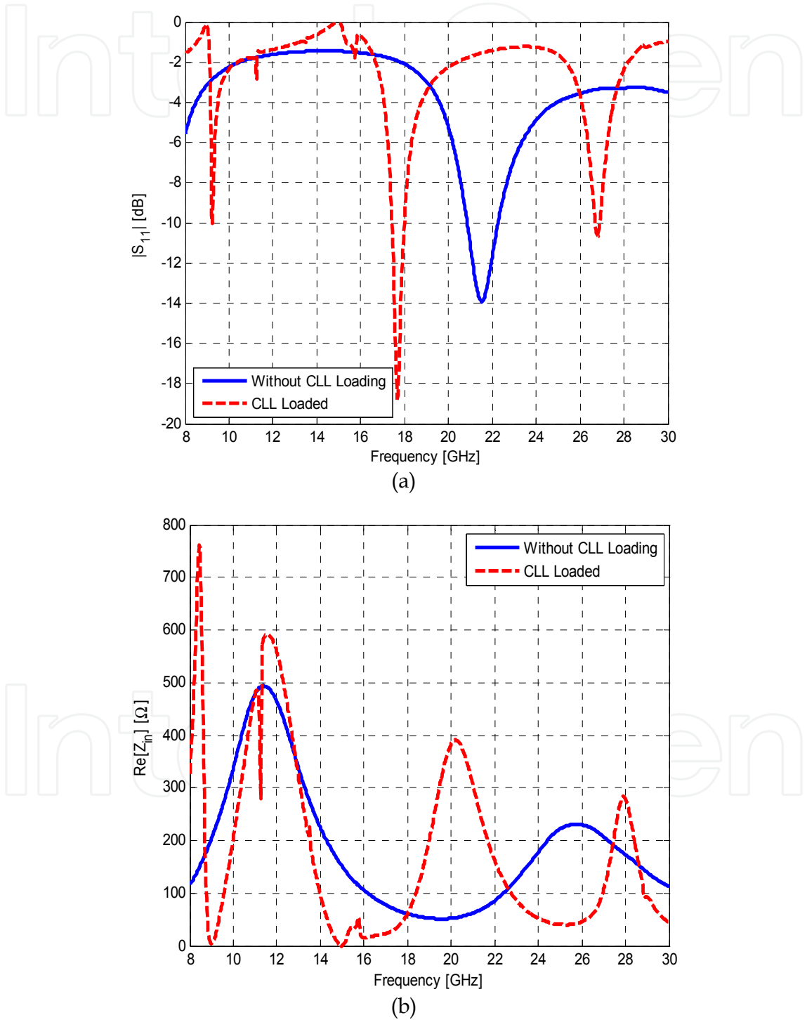
Fig. 13. (a) simulated reflection coefficient, and (b) Input Impedance of the CLL loaded and unloaded wire dipole antennas.
