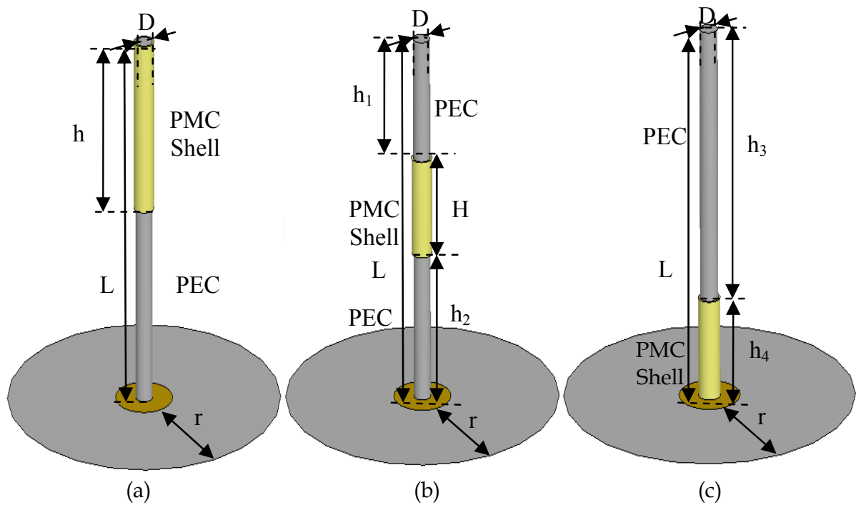
Fig. 1. Three ideal models of PMC loaded monopole antennas, (a) case I, (b) case II, and (c) case III: L=7.5\text{mm} , D=0.5\text{mm} and h=3.5\text{mm} , h_1=2.5\text{mm} , h_2=3\text{mm} , H=2\text{mm} , h_3=5.5\text{mm} , h_4=2\text{mm} , and r=4\text{mm} . From (Jafargholi et al., 2010), copyright © 2010 by the Institute of Electrical and Electronics Engineers (IEEE).
