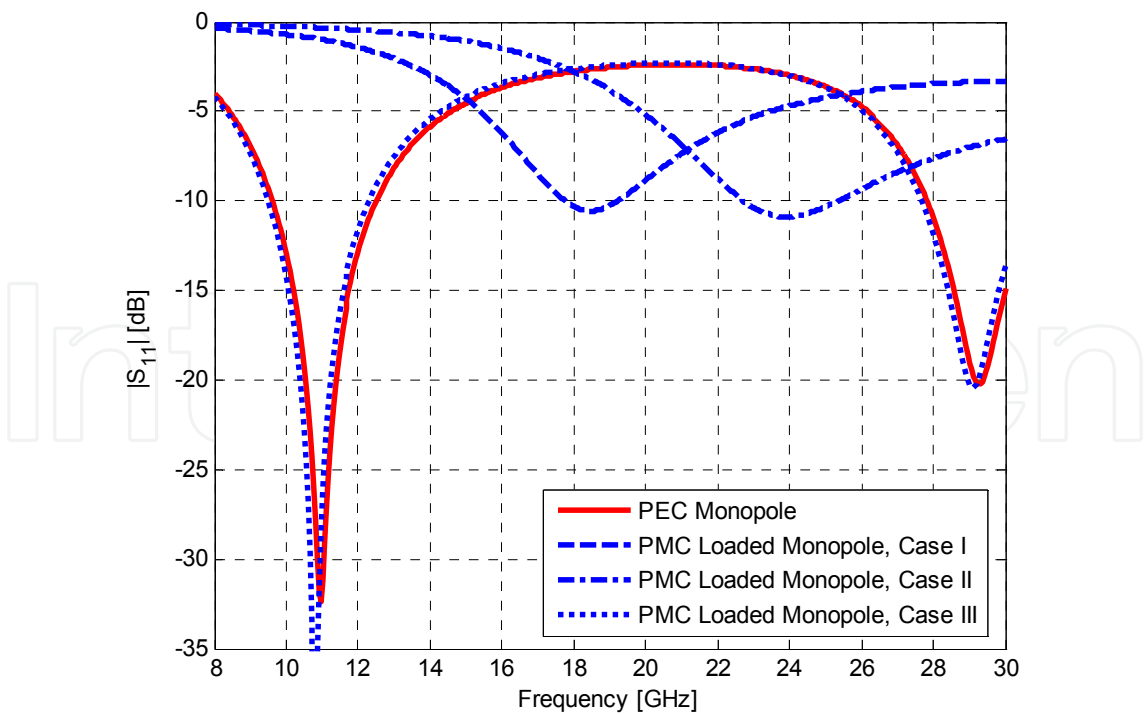
Fig. 2. Reflection coefficient of monopole antennas with and without PMC cover. From (Jafargholi et al., 2010), copyright © 2010 by the Institute of Electrical and Electronics Engineers (IEEE).
