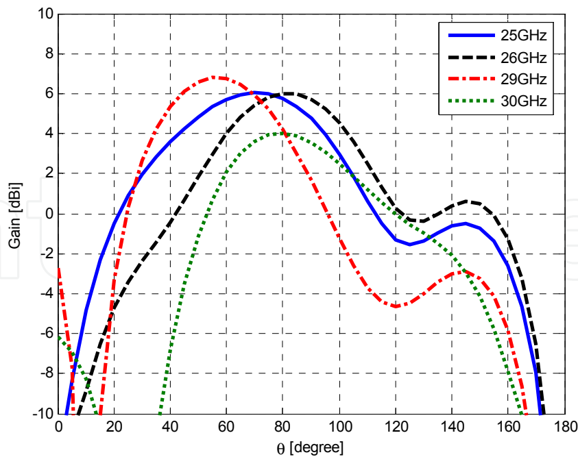
Fig. 10. Radiation patterns of the CLL loaded monopole antenna versus frequency at \varphi=0^{\circ} . From (Jafargholi et al., 2010), copyright © 2010 by the Institute of Electrical and Electronics Engineers (IEEE).
