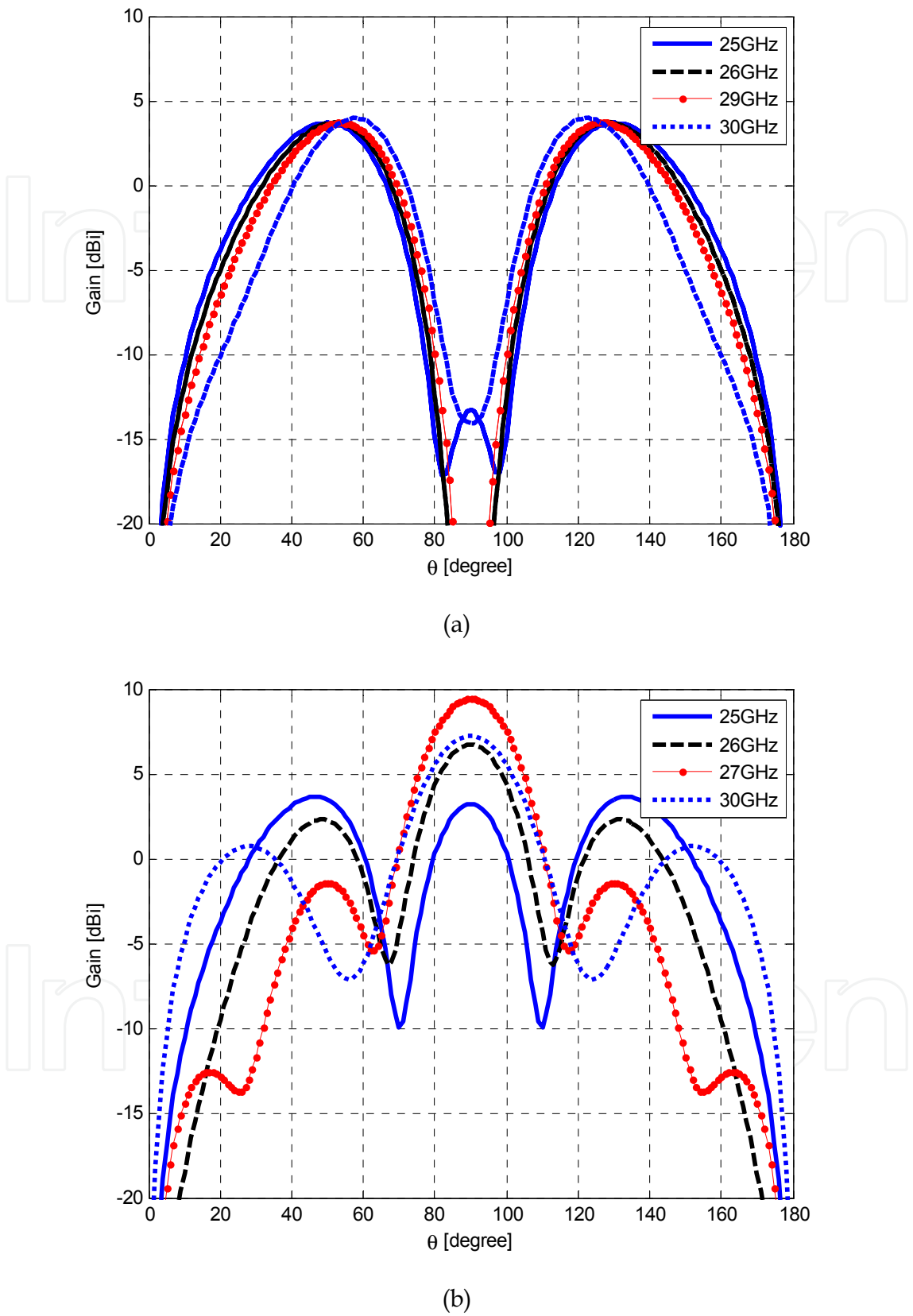
Fig. 16. Radiation patterns of (a) conventional wire dipole antenna, and (b) the CLL loaded dipole antenna versus frequency at \varphi=0^\circ .
