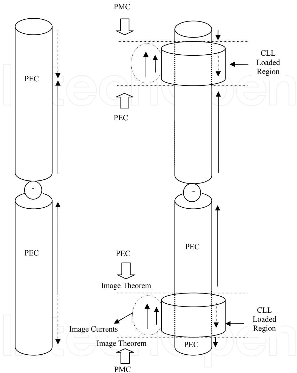
Fig. 15. Conceptual schematics of the conventional (left) and CLL loaded dipole (right).
