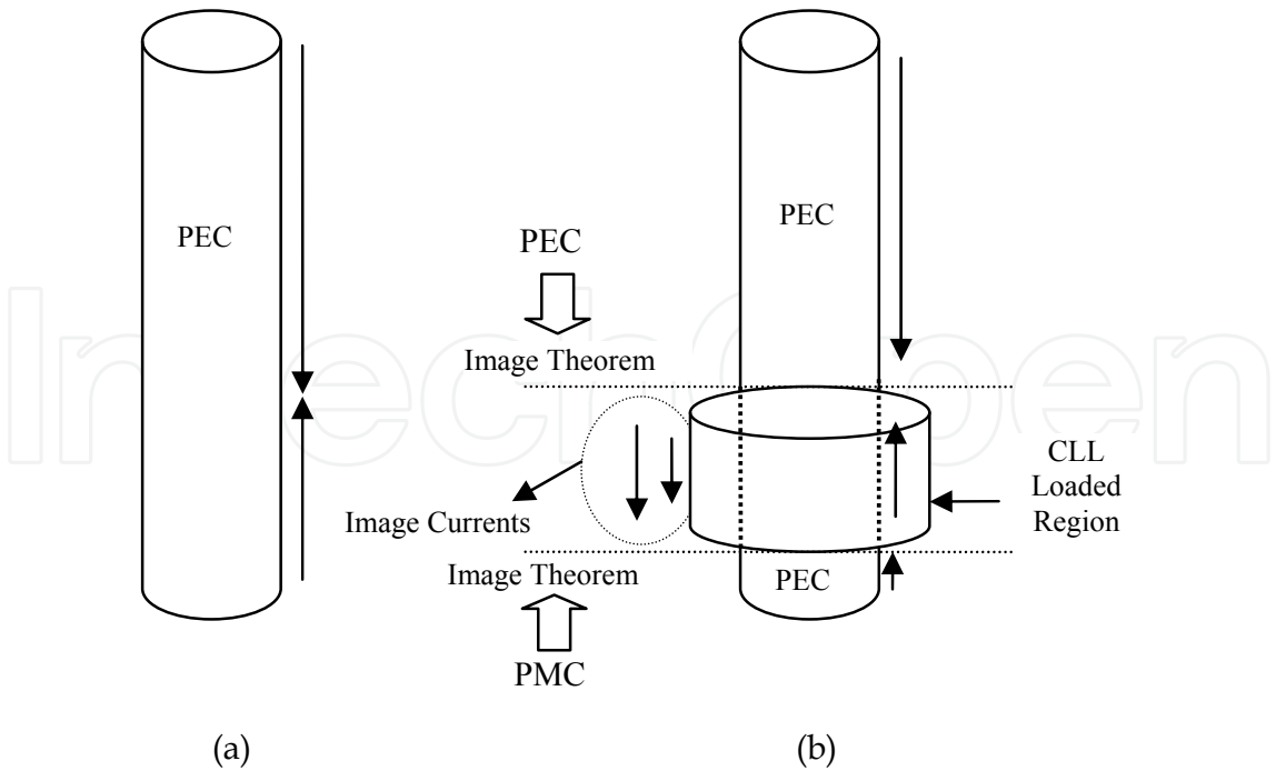
Fig. 8. Conceptual schematics of the (a) conventional and (b) PMC-loaded monopoles. From (Jafargholi et al., 2010)], copyright © 2010 by the Institute of Electrical and Electronics Engineers (IEEE).
