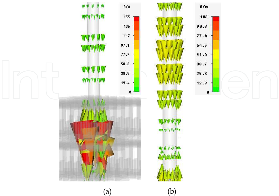
Fig. 7. Surface current densities on the (a) CLL loaded monopole and (b) unloaded monopole at f= 25\text{GHz} . From (Jafargholi et al., 2010), copyright © 2010 by the Institute of Electrical and Electronics Engineers (IEEE).
