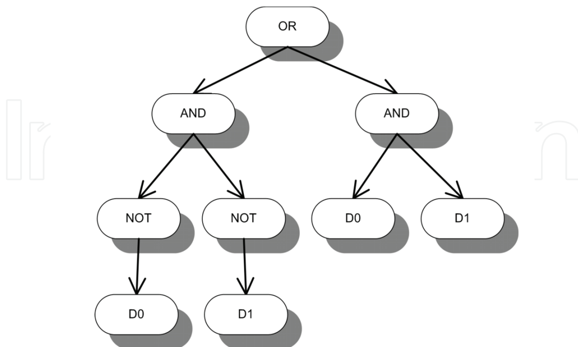
Fig. 2. S-expression: tree architecture.
