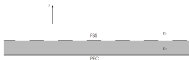
Fig. 6. Cross section view of a single layer FSS with dielectric substrate on ground plane.
