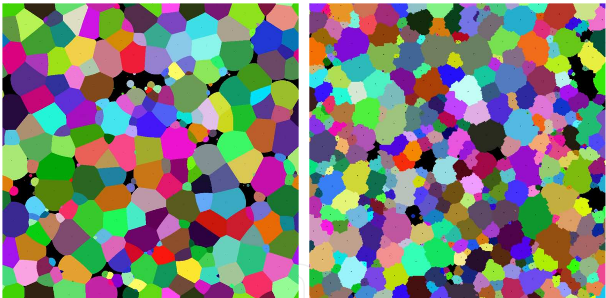
(c) the crown shape projection on the ground in the Crown Plastic SORTIE simulations. (d) the crown shape projection on the ground in LES model simulations.
