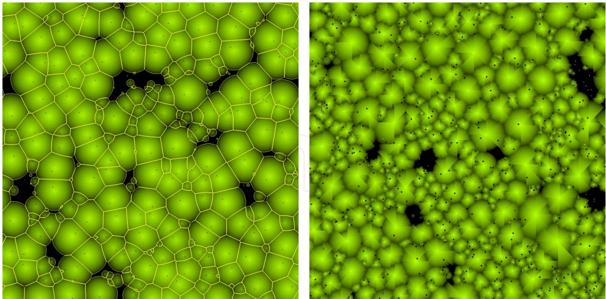
(a) Canopy simulated with the Crown Plastic SORTIE model. (b) Canopy simulated with the LES model.
