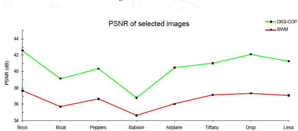
Fig. 10. PSNR values of selected watermarked images with \alpha = 40
