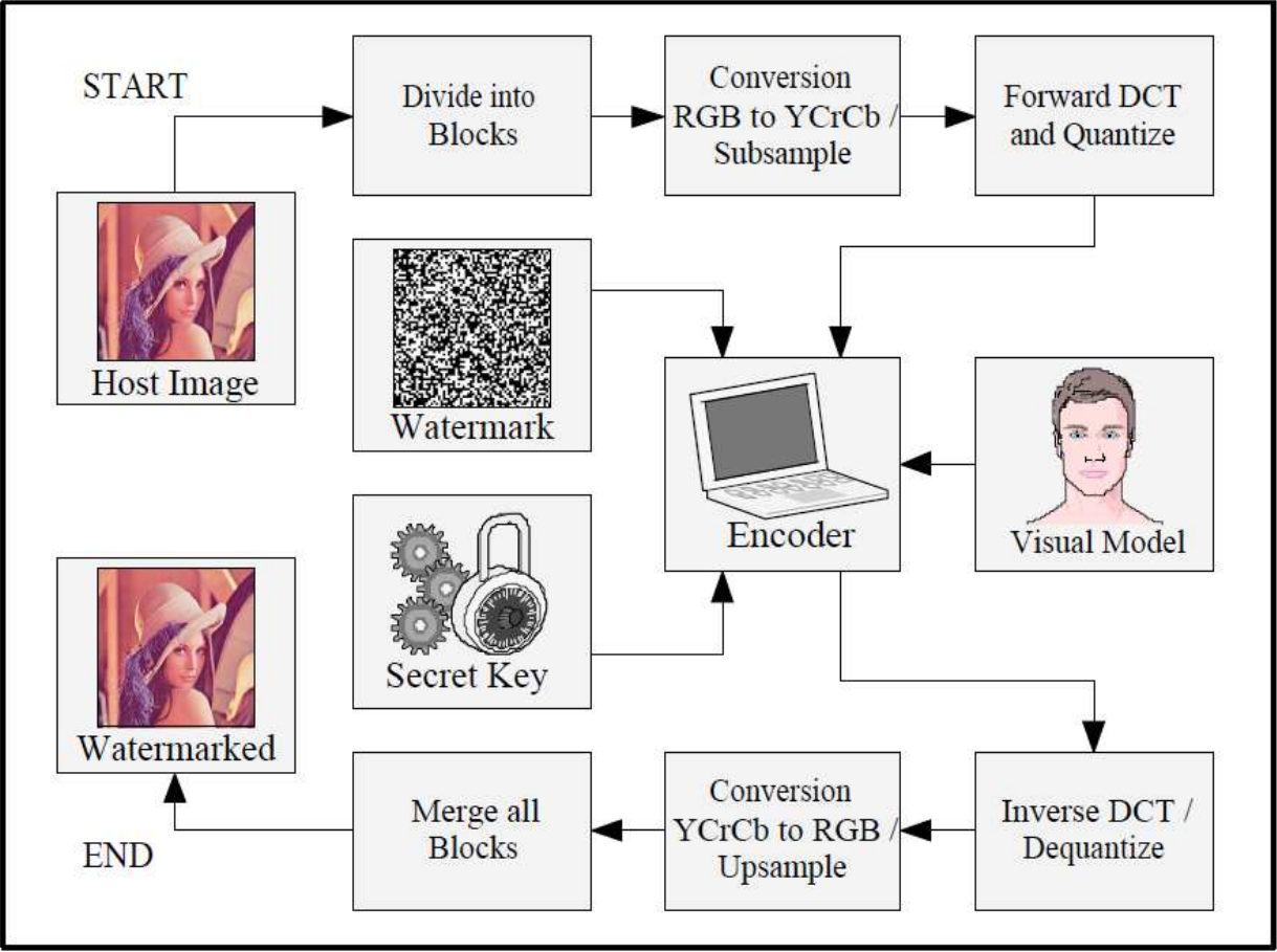
Fig. 7. Proposed watermark encoding diagram
