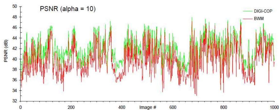
Fig. 9. PSNR values of 1000 watermarked images with \alpha = 10
