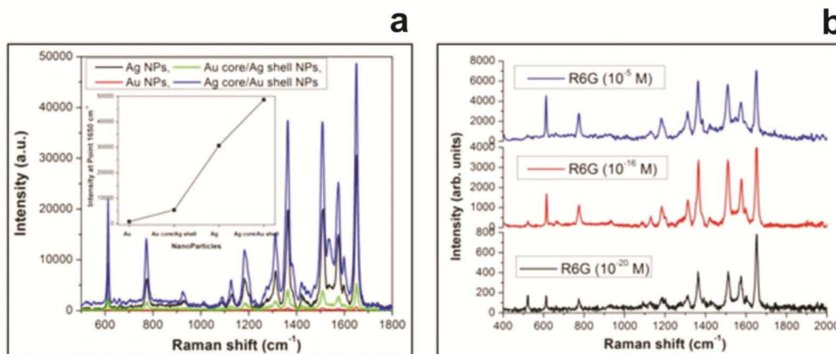
Fig. 15. a) R6G [ 10^{-12} M], absorbed on the silver, gold, Ag/ Au and Au/ Ag structures. Raman signal increases from Au, Au core/ Ag shell, Ag and Ag core/ Au shell; b) 3. SERS spectra acquired from 10^{-5} , 10^{-16} and 10^{-20} M R6G, absorbed on the silver nanostructures.
