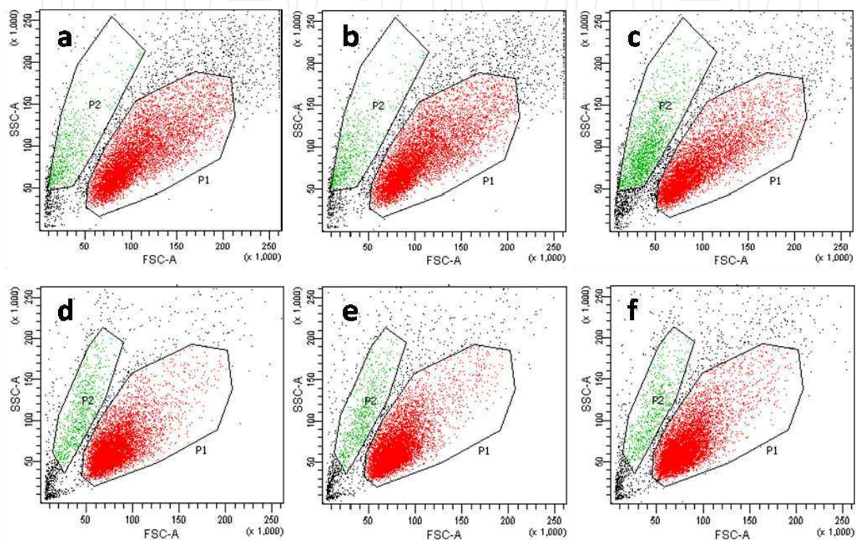
Fig. 4. Density plot of HCT116 (a, b, c) and THP1 (d, e, f) cell lines. Gate P1 shows cell viability %. a) HCT116 cells control without NPNPs, (P1 79%). b) HCT116 cells incubated with not annealed NPNPs (P1 78%). c) HCT116 cells incubated with annealed NPNPs (P1 68%). d) THP1 cells control without NPNPs (P1 83%). e) THP1 cells incubated with not annealed NPNPs (P1 82%). f) THP1 cells incubated with annealed NPNPs (P1 82%).
