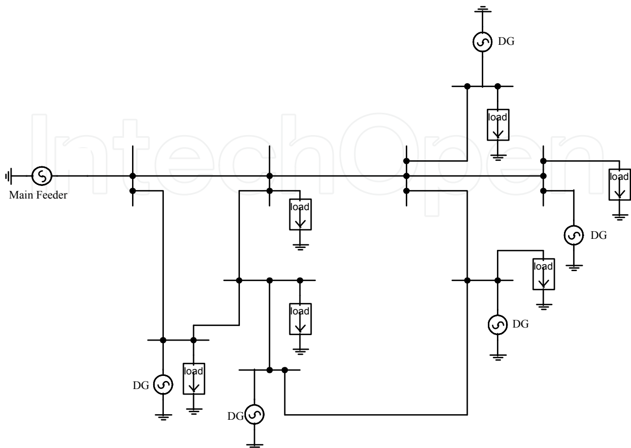
Fig. 1. Sample Distribution System with DG
