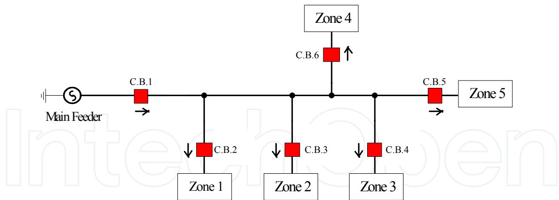
Fig. 2. Distribution system divided into several zones
