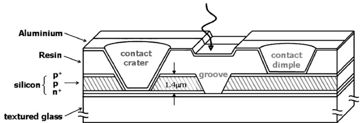
Fig. 9. Key features of the crystalline silicon on glass (CSG) technology . (Bagnall and Boreland, 2008)
