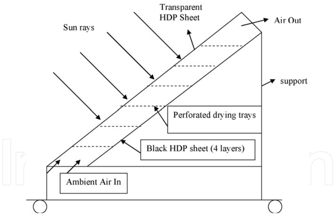
Fig. 8. Multiple-shelf portable solar drier.
