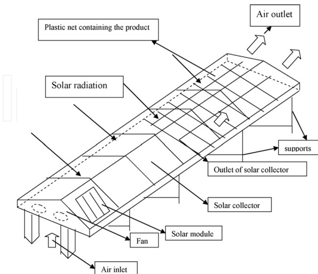
Fig. 7. Solar tunnel dryer.
