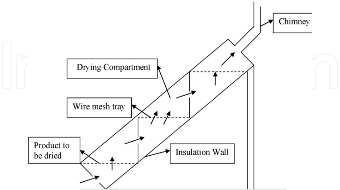
Fig. 9. Staircase solar drier.
