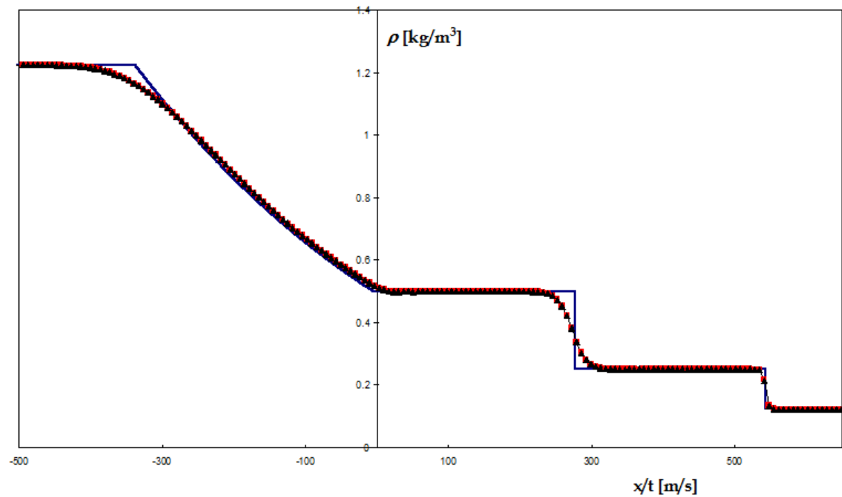
Fig. 6. One-dimensional HLLC method. Blue line: theoretical solution. Red squares: exact solvers. Black triangles: approximate solver
