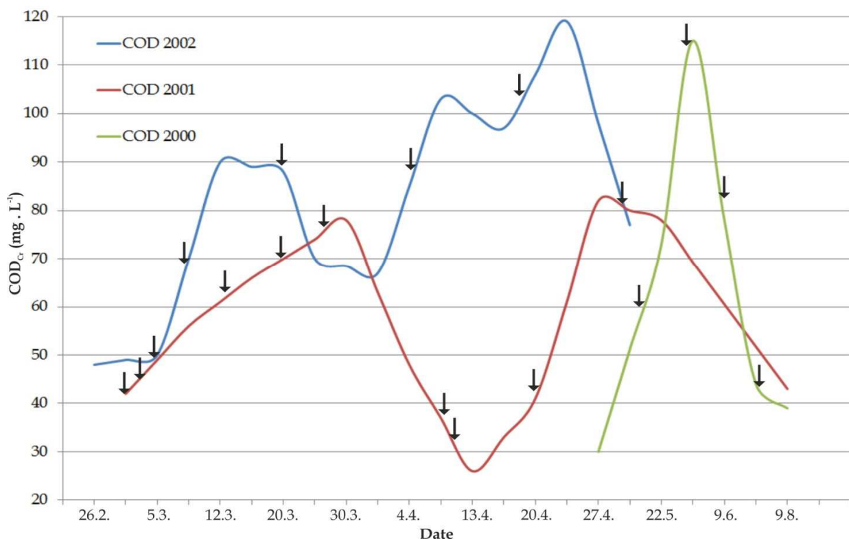
Fig. 5. Variation values of chemical oxygen demand (COD Cr ) during application of pig slurry into the ponds. Level of total doses 16 \text{ kg} \cdot \text{m}^{-2} (2001, 2002) and 0.10 \text{ kg} \cdot \text{m}^{-2} (2000). (Arrows indicate term of application of pig slurry)
