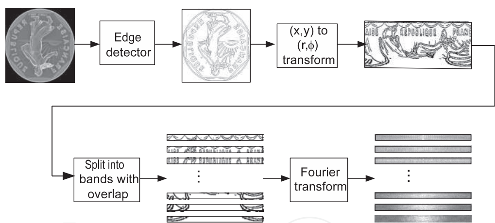
Fig. 4. Processing for rotational invariance
