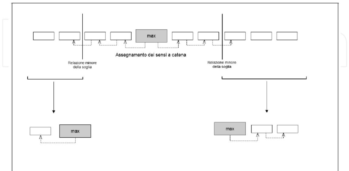
Fig. 4. The SenseDisambiguator recursive procedure
