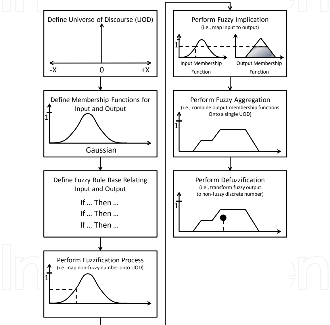
Fig. 3. Flowchart for fuzzy logic analysis based on Mamdani’s fuzzy inference method (Symans & Kelly, 1999)
