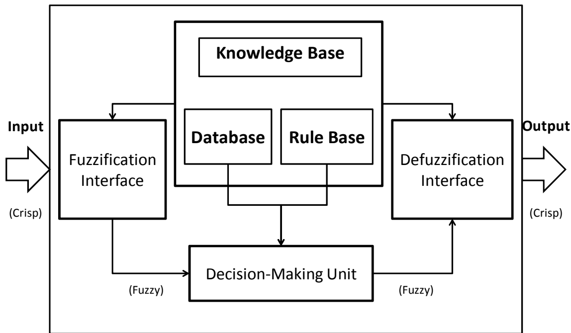
Fig. 2. Fuzzy Inference System (FIS)
