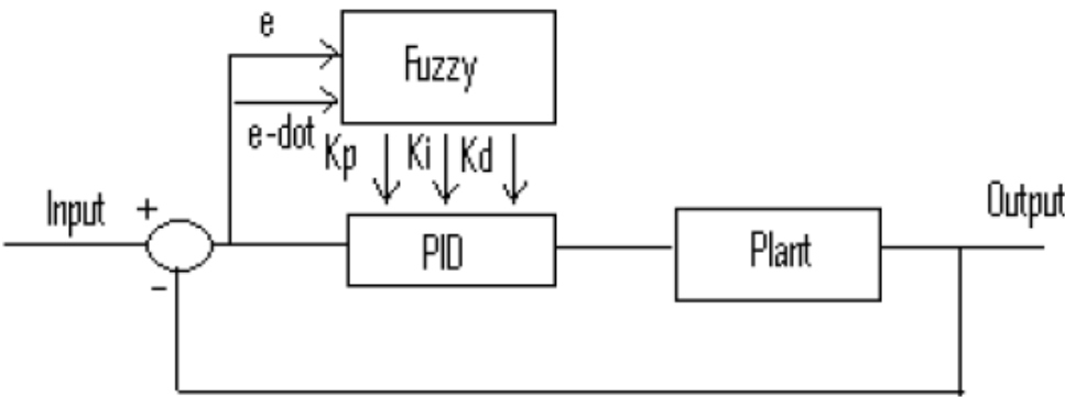
Fig. 15. Structure of the Fuzzy-tuned PID controller
