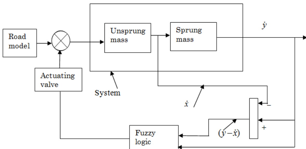
Fig. 6. Block diagram representation of the control system
