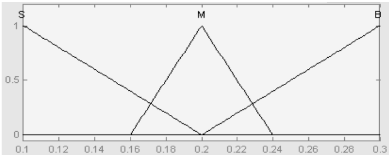
Fig. 21. Membership function for output gain Ki
