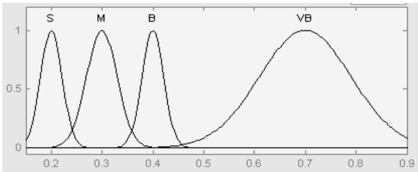
Fig. 19. Membership function for output gain Kd
