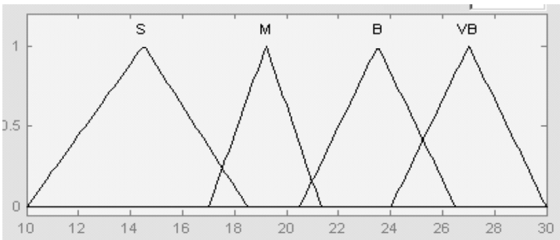
Fig. 17. Membership function of output, Kp
