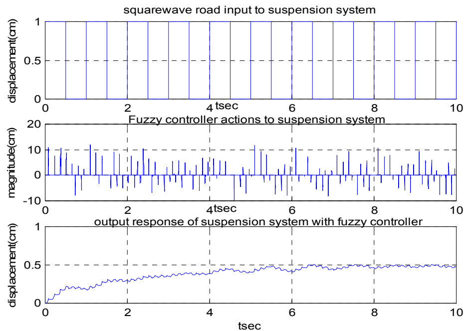
Fig. 10. Suspension controller responses with square-wave input
