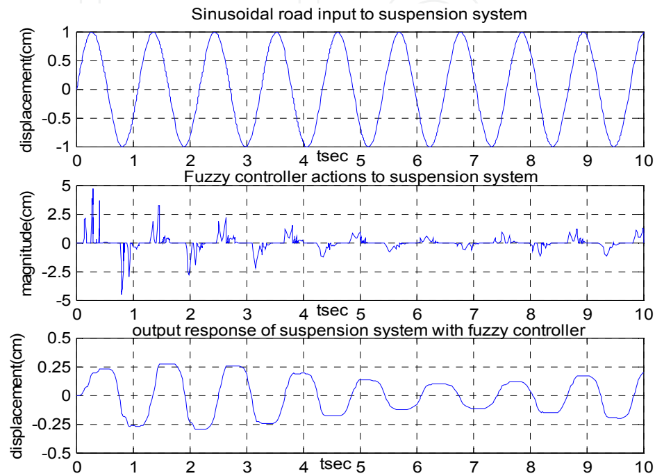
Fig. 9. Suspension controller responses with sinusoidal input
