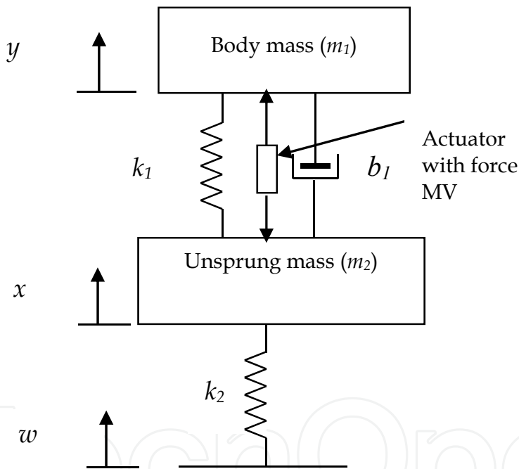
Fig. 4. Modeling of quarter-car suspension system
