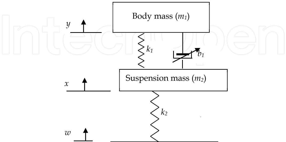
Fig. 3. Quarter-Car Model
