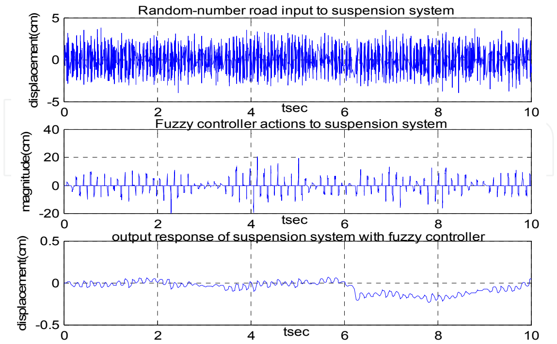
Fig. 12. Suspension controller response with random number input
