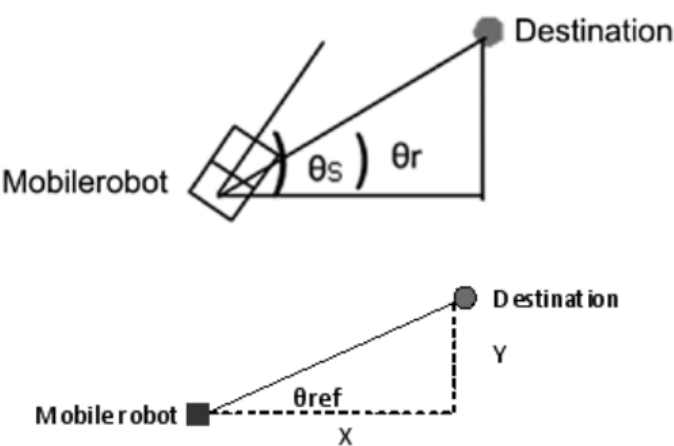
Fig. 23. Autonomous Robot with parameters defined
