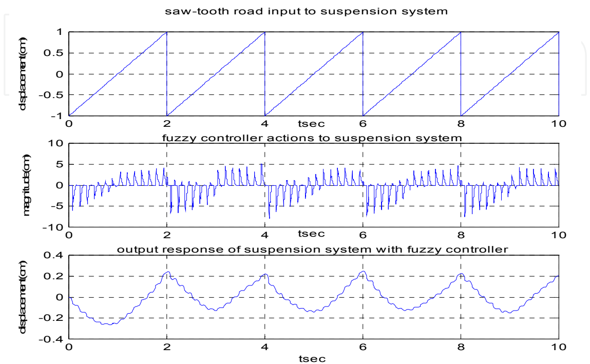
Fig. 11. Suspension controller responses with saw tooth wave input
