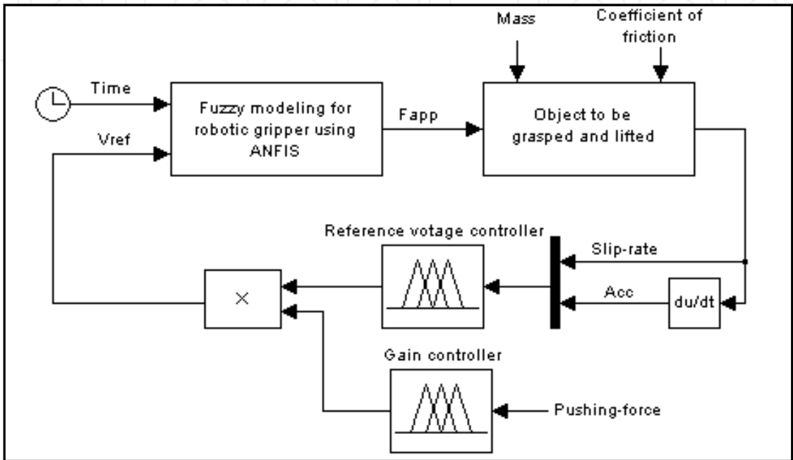
Fig. 19. Block diagram of the first scheme controller
