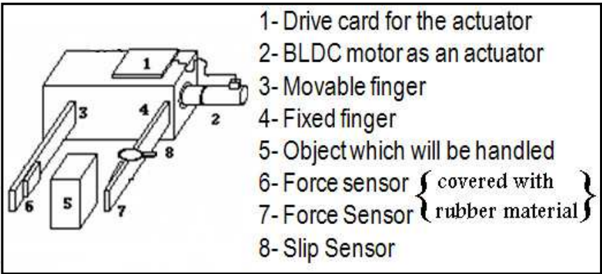
Fig. 4. Gripper configuration.
