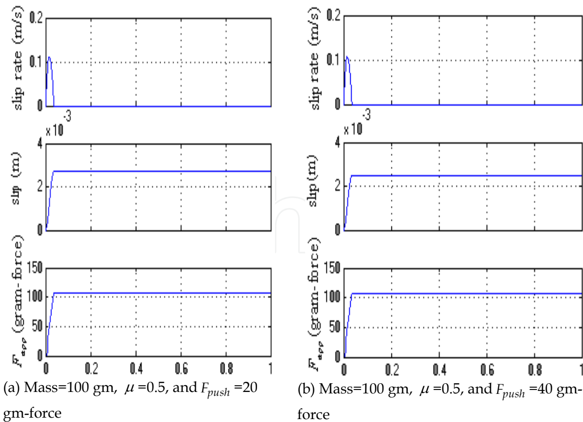
Fig. 25. Slippage parameters and applied force.
