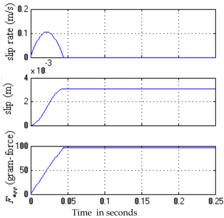
Fig. 16. Object simulation results when Mass=100 gm and \mu=0.5 .
