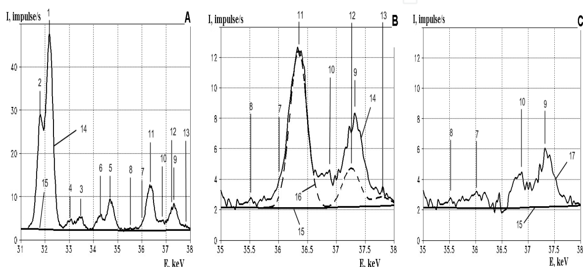
Fig. 3. Spectral segment corresponding to the K-lines of Ba, La, Ce, Pr, and Nd for the SGD-1A (gabbro-essexite) reference standard: (A) general spectrum view; (B) detailed interpretation of the spectrum for Pr and Nd with the simulation of the K_{\beta} components of the Ba and La lines; (C) the spectrum after the subtraction of the K_{\beta} components. The spectral lines: (1) Ba K_{\alpha 1} ; (2) Ba K_{\alpha 2} ; (3) La K_{\alpha 1} ; (4) La K_{\alpha 2} ; (5) Ce K_{\alpha 1} ; (6) Ce K_{\alpha 2} ; (7) Pr K_{\alpha 1} ; (8) Pr K_{\alpha 2} ; (9) Nd K_{\alpha 1} ; (10) Nd K_{\alpha 2} ; (11) Ba K_{\beta 1} ; (12) Ba K_{\beta 2} ; (13) La K_{\beta 1} . (14) the original spectrum obtained by the energy dispersive analyzer; (15) approximation of the background radiation; (16) simulation of the K_{\beta} components of the Ba and La lines; (17) true spectrum after the subtraction of the K_{\beta} components.
