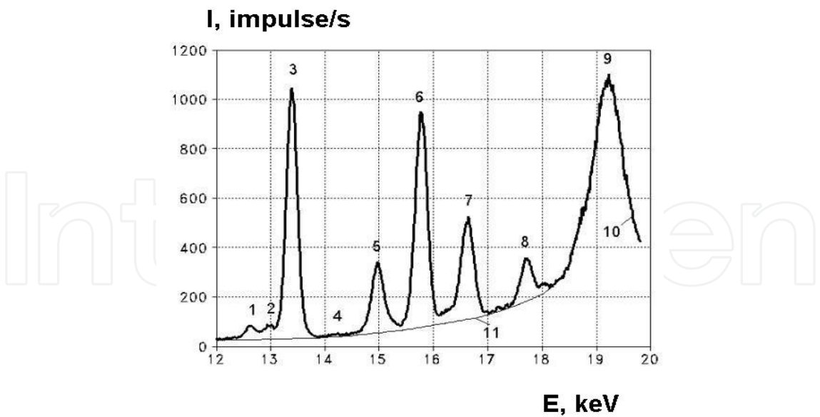
Fig. 1. Part of the SSC SG-1A spectrum from Pb L_{\beta} to Zr K_{\beta} (EX-6500 analyzer, X-ray fluorescence method). Position of characteristic lines on the curve: (1) Pb L_{\beta\gamma} (2) Th L_{\alpha'} (3) Rb K_{\alpha'} (4) Sr K_{\alpha'} (5) Y K_{\alpha} + Rb K_{\beta\gamma} (6) Zr K_{\alpha'} (7) Nb K_{\alpha} + Y K_{\beta\gamma} (8) Zr K_{\beta\gamma} (9) incoherent scattering Rh K_{\alpha} (material of anode), (10) distribution given by multichannel analyzer, (11) approximation of background radiation.
