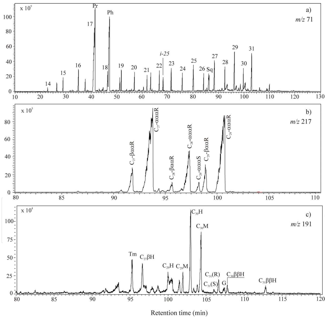
for peak assignments, see legends, Figs. 3, 4 and 7 Fig. 6. GC-MS ion fragmentogram of n -alkanes and isoprenoids, m/z 71 (a), steranes, m/z 217 (b) and terpanes, m/z 191 (c) representative for sediments from depth interval 360–400 m
