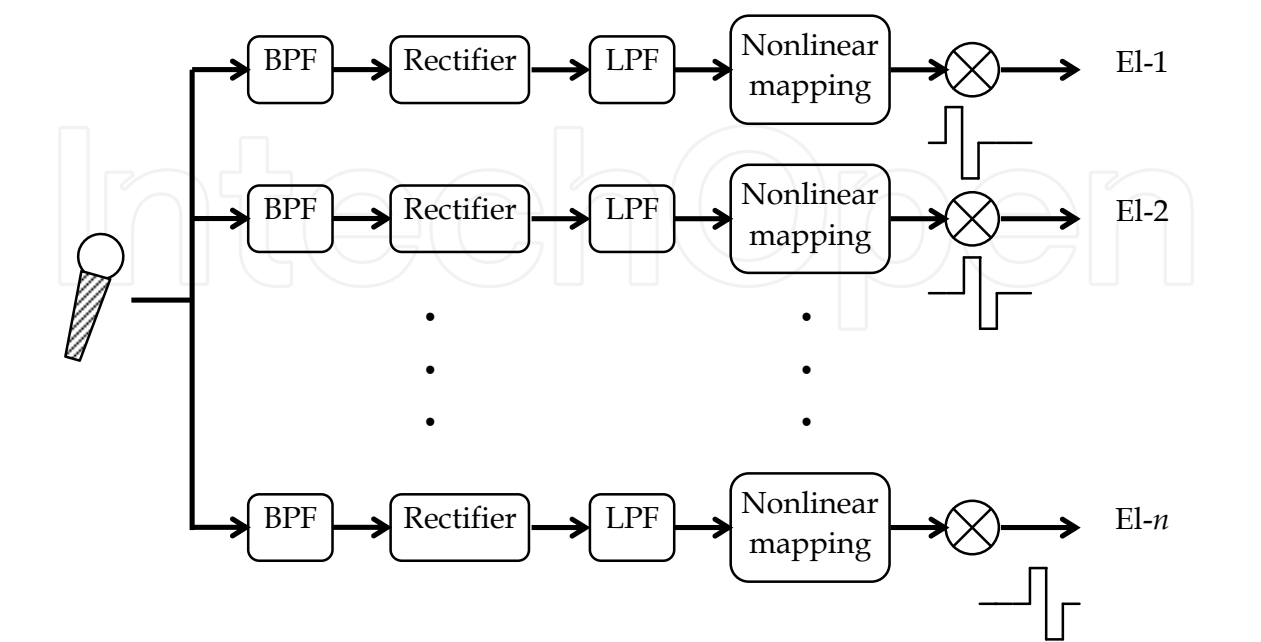
Fig. 5. A block diagram of the CIS stimulating strategy.
