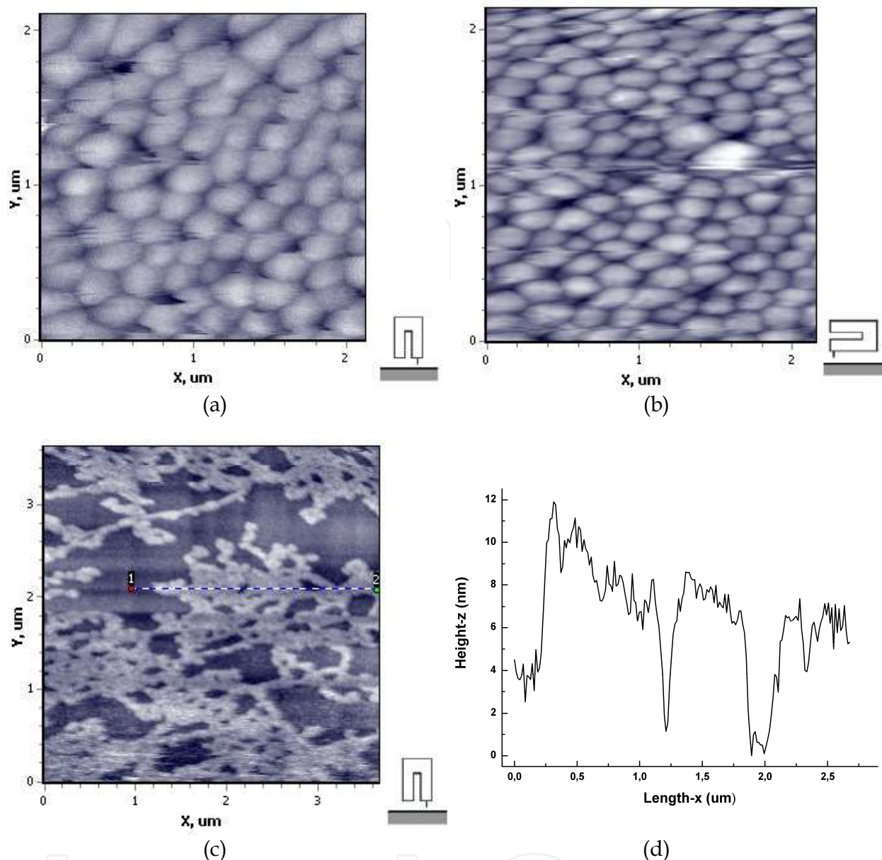
Fig. 10. Topography images of (a, b) alumina \text{Al}_2\text{O}_3 , (c) “non-rigid” sample PVP in the shear-force and intermittent contact modes using Q-control feedback ( Q < 2500 ). The dimensions of images is noted in the figure. A line profile from 1 to 2 in (c) is show in figure (d)
