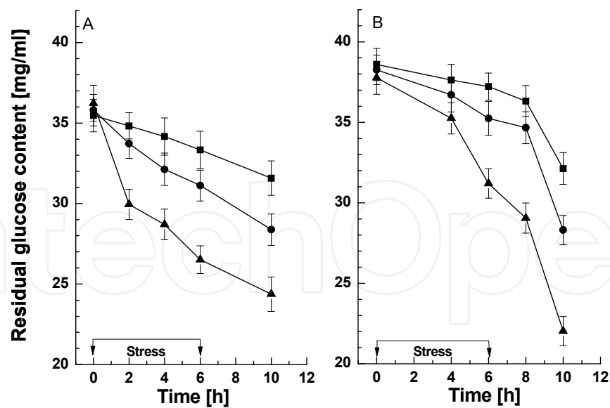
Fig. 2. Glucose consumption in Penicillium sp. 161 (A) and A. glaucus 363 (B) during cold shock and following recovery period. (▲) - growth at optimal temperature; (■)- downshift from optimal temperature to 4°C; (●) - downshift from optimal temperature to 10°C. Bars represent SD of means. The effect of treatment was significant for the temperature treatment ( P \leq 0.05 )
