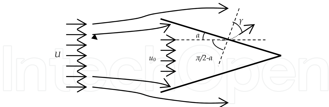
Fig. 2. Sketch of flow through a conical net with taper angle \alpha and filtration efficiency F = u_0/U , the angle \gamma describes streamline deflection through the net wall ("cf." from Gjøsund and Enerhaug, 2010).
