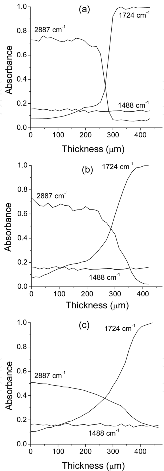
Fig. 6. Plots of the peak intensity of the P(BA-co-BT) C=O, PEO C-H, and TDP C=C absorptions along the thickness direction of the resulted films after annealed for (a) 4 hours, (b) 8 hours, and (c) 12 hours.
