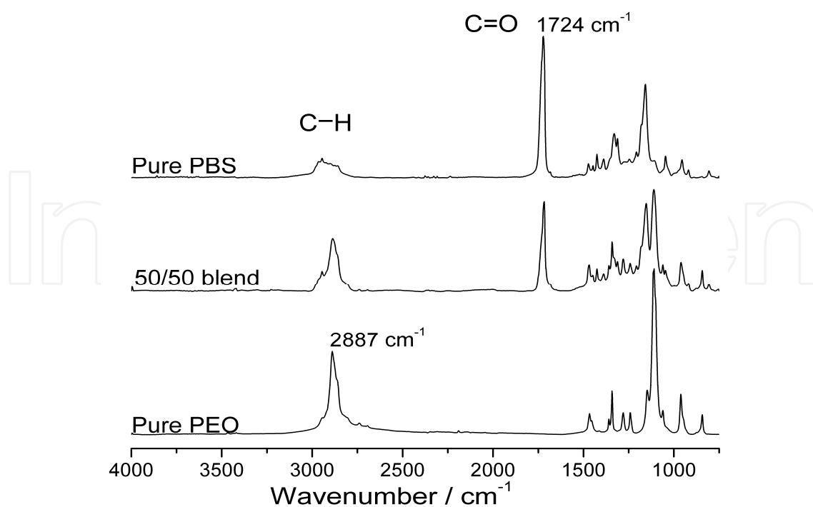
Fig. 1. ATR-FTIR spectra of pure PBS, PEO, and 50/50(wt%/wt%) PBS/PEO binary blend observed at room temperature.
