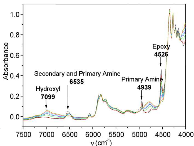
Fig. 7. Time evolution of FTnIR spectra during the isothermal curing at 70 °C of the stoichiometric HDGEBA/poly(3-aminopropylmethyl)siloxane system.
