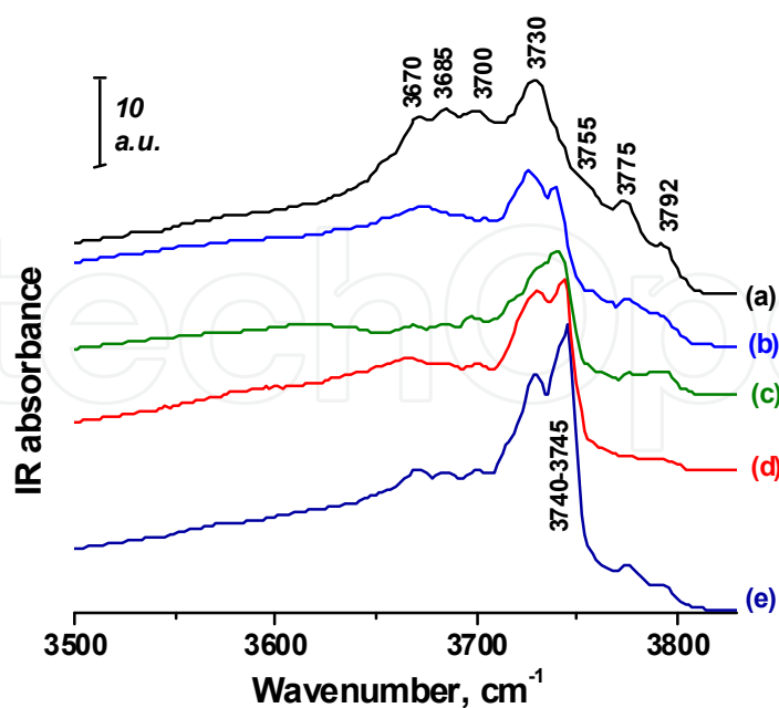
Fig. 8. FTIR spectra of hydroxyl groups for \gamma\text{-Al}_2\text{O}_3 calcined at 550 ^{\circ}\text{C} (a) and of 1.5% \text{SiO}_2/\gamma\text{-Al}_2\text{O}_3 (b), 5% \text{SiO}_2/\gamma\text{-Al}_2\text{O}_3 (c), 7% \text{SiO}_2/\gamma\text{-Al}_2\text{O}_3 (d), 10% \text{SiO}_2/\gamma\text{-Al}_2\text{O}_3 (e) calcined at 450 ^{\circ}\text{C} . The samples were outgassed at 450 ^{\circ}\text{C}
