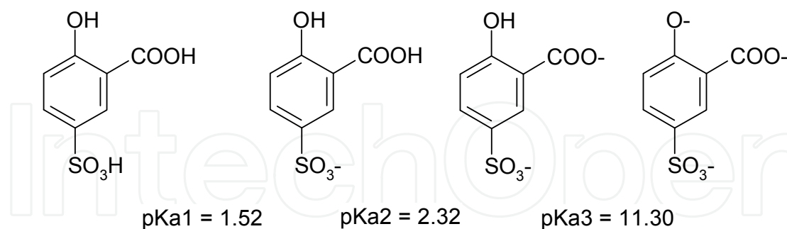
Fig. 8. Equilibrium constants for the deprotonation of 5-SSA (Panak, 1996).
