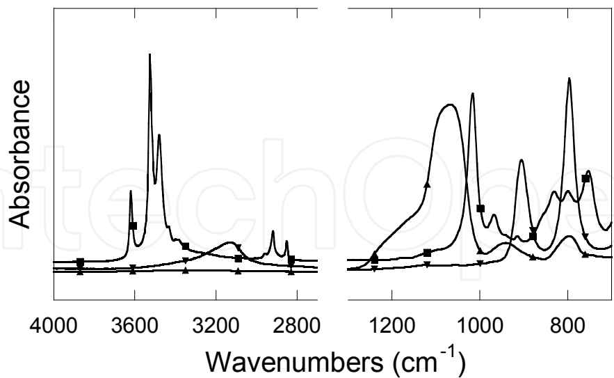
Fig. 3. Spectra of solids as dried layer on an ATR element: silica (▲), gibbsite (■), goethite (▼) below 890 cm -1 (Lefèvre et al., 2006). To be able to record spectra at lower wavenumbers, heavy water (D 2 O) can be used because the absorption bands are shifted by a factor of ca. 1.4 to lower wavenumbers. Thus, a good signal can be obtained for bands located between 850 and 950 cm -1 (Lefèvre et al., 2008) using the same 25-reflection crystal. It can be useful to avoid interferences with bands around 1650 cm -1 since D 2 O bending is located at 1209 cm -1 (Venjaminov and Prendergast, 1997).
