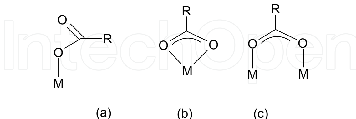
Fig. 4. Surface complexes between a monoacid and a metal oxide: (a) monodentate, (b) mononuclear bidentate and (c) binuclear bidentate
