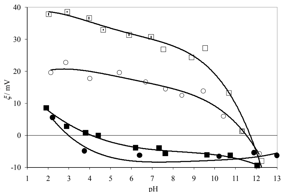
Fig. 10. Zeta-potentials of gibbsite particles in the absence ( \square, \circ ) and in the presence ( \blacksquare, \bullet ) of 5-SSA. Ionic strength was controlled by NaCl: 10^{-1} \text{ mol.dm}^{-3} (circles) and 10^{-2} \text{ mol.dm}^{-3} (squares). Temperature was 25^\circ\text{C} .
