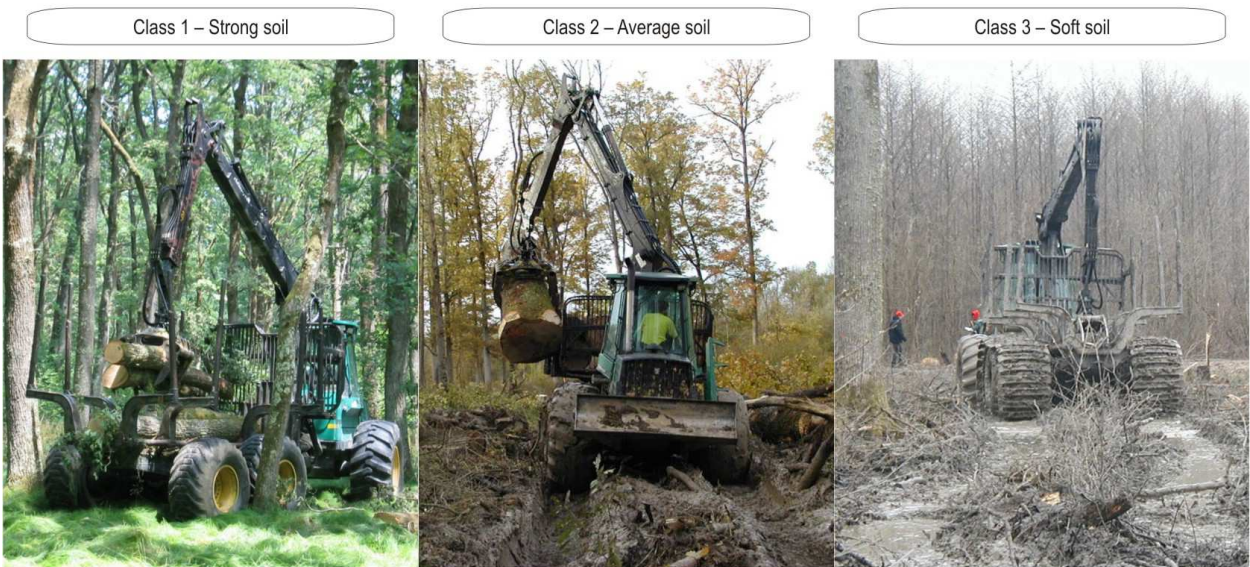
Fig. 2. Soil strength classes
