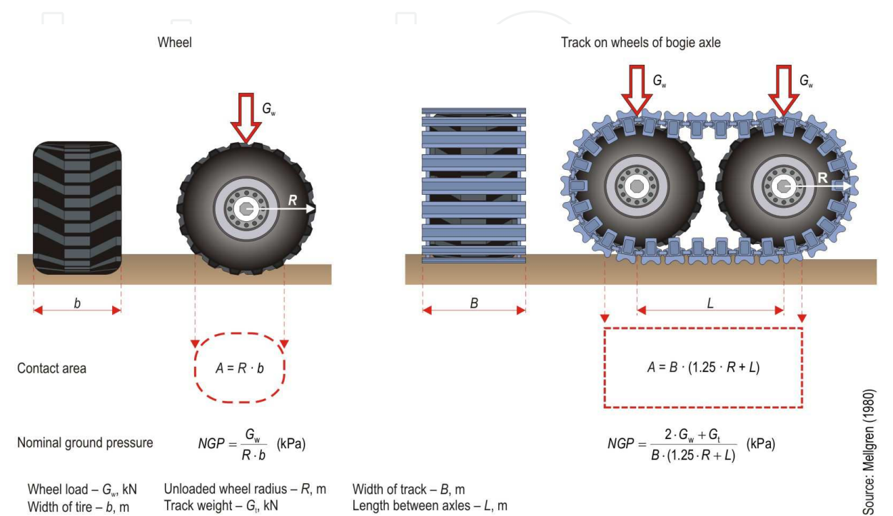
Fig. 3. Calculation of Nominal Ground Pressure
