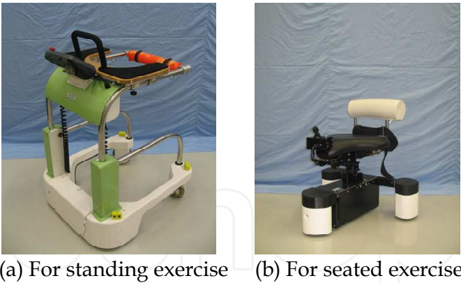
Fig. 2. Omnidirectional walkers.
