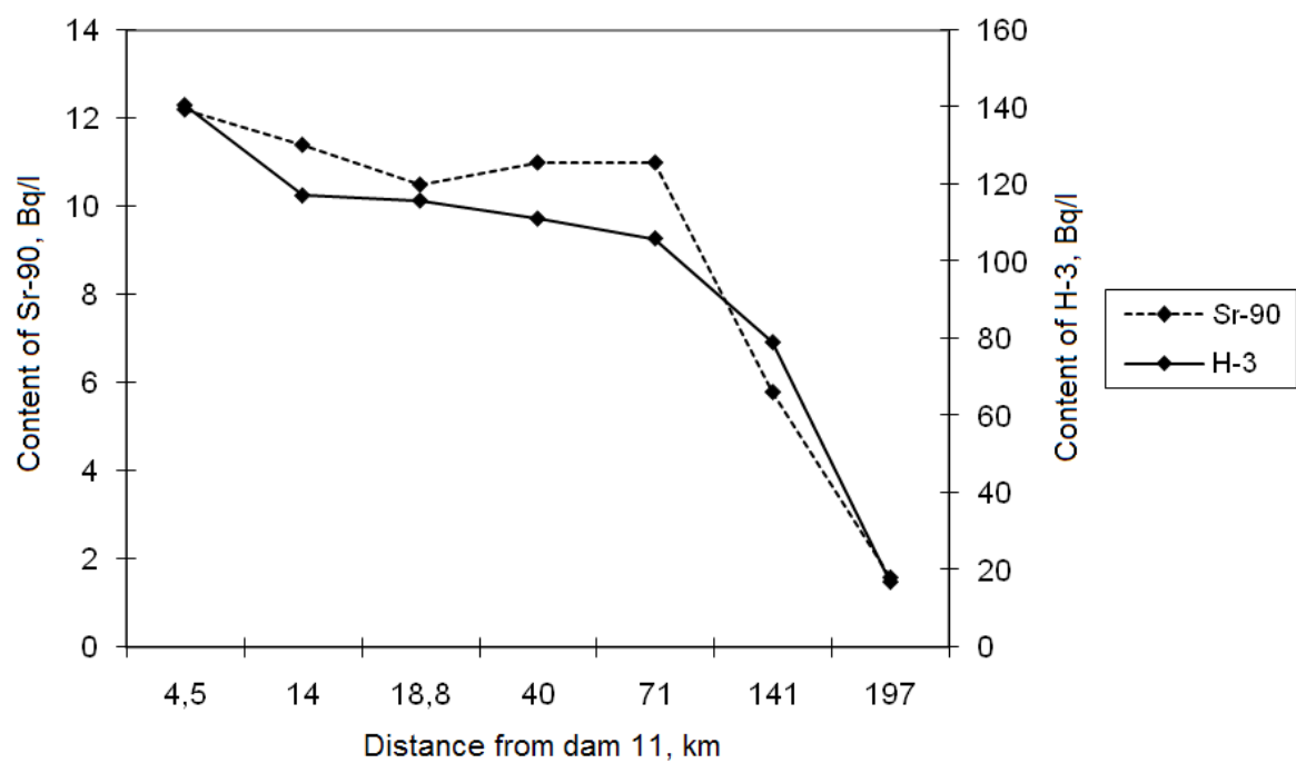
Fig. 6. Content of 90 Sr and 3 H in water of the Techa River
