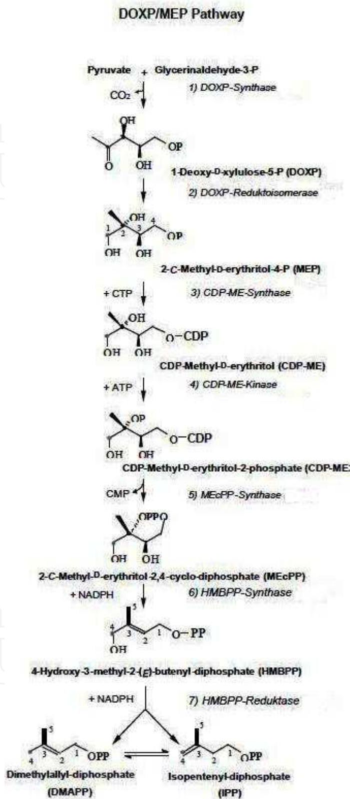
Fig. 3. Scheme of 1-deoxy-D-xylulose-5-phosphate/ methyl-D-erythrithol (DOXP/MEP pathway). The enzymes of both pathways are numbered. MEP/DOXP pathway for isopentenyl diphosphate (IPP) and isoprenoid biosynthesis
