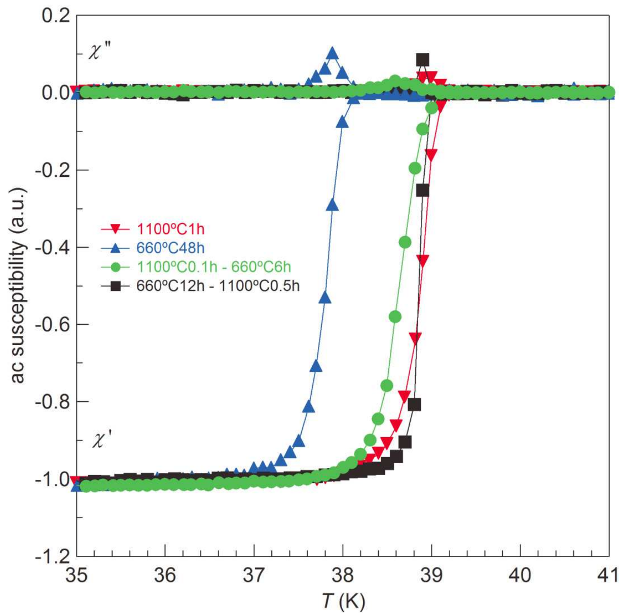
Fig. 3. The real and imaginary components of ac susceptibility with f = 76.97 Hz, \mu_0 H_{ac} = 10 \mu T, and \mu_0 H_{dc} = 0 T for Mg diffusion processed samples via four major sintering conditions that are 1100 °C for 1 hour, 660 °C for 48 hours, 1100 °C for 0.1 hour followed by second sintering at 660 °C for 6 hours, and 660 °C for 12 hours followed by second sintering at 1100 °C for 0.5 hour.
