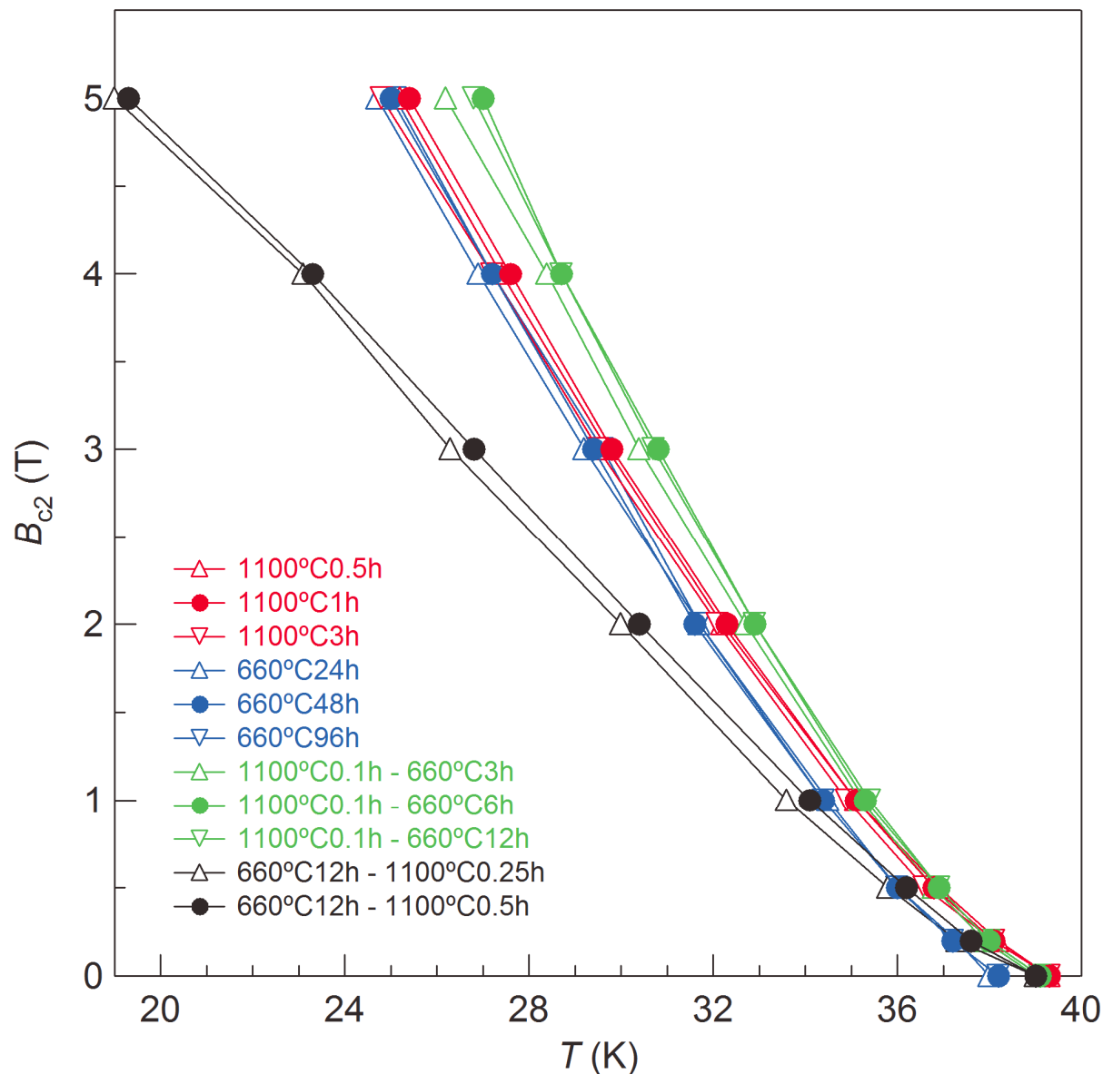
Fig. 4. The temperature dependence of B c2 derived from ac susceptibility with f = 76.97 Hz, \mu_0 H_{ac} = 10 \mu T, and \mu_0 H_{dc} = 0, 0.2, 0.5, 1, 2, 3, 4, and 5 T for MgB 2 samples sintered via various conditions.
