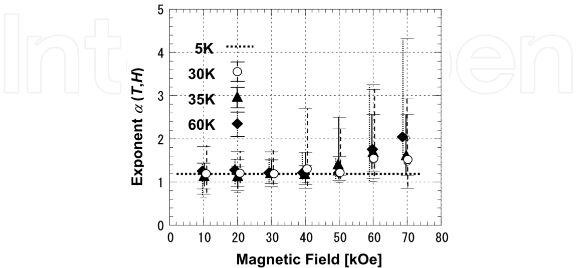
Fig. 12. Magnetic field dependence of the exponent \alpha(T,H) in the I - V characteristics at 5, 30, 35, 60 K with V=AI^\alpha .
