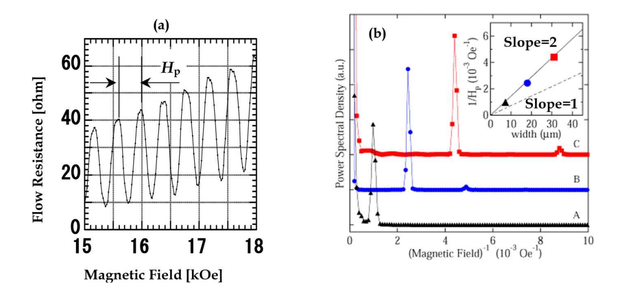
Fig. 6. (a) Periodic oscillations in JV flow-resistance; enlarged part of Fig.3. (b). (b) Power spectrum of the periodic oscillations in fast Fourier transform on samples A, B and C. Inset shows width ( w ) dependency of the inverse of H_p . The broken and solid lines represent 1/H_0(w) and its double, respectively.
