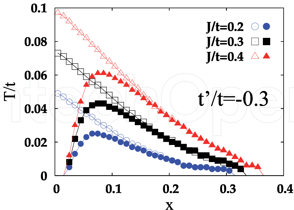
Fig. 2. (color online). Variation of phase diagram with Heisenberg coupling strength J for t'/t = -0.3 .
