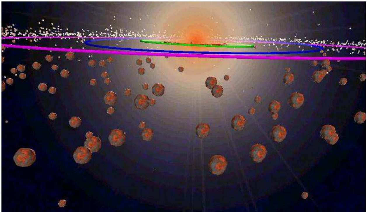
Fig. 10. Visualization outputs from research results in Astrophysics science simulations. Dynamical evolution of O-orth cloud - thirrh position.
