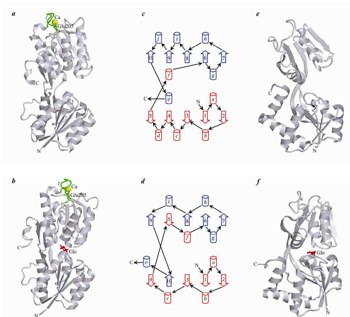
Fig. 1. Spatial pattern of PBP of group I and group II. Tertiary structures of GGBP (a) and its complex with glucose GGBP/Glc (b), representing group I, are shown. The residues of the Ca-binding site are shown in green, including the loop in the protein's C-terminal domain (residues 134-142; 1) and Glu 205. Calcium is represented as a yellow sphere. The structures of group II GlnBP (e) and its complex with glutamine GlnBP/Gln (f) are shown. In both cases, the ligand (glucose or glutamine) is represented as a red stick union. The structures were created based on PDB data (Dutta et al., 2009); PDB codes 2GBP.ent15 (Vyas et al., 1988), 2FWO.ent16 (Borrok et al., 2007), 1GGG (Hsiao et al., 1996) and 1WDN (Sun et al., 1998) using the graphical software VMD (Hsin et al., 2008) and Raster 3D (Merritt & Bacon, 1977). The topology of group I (c) and group II (d) proteins is drawn with \beta -strands and \alpha -helices indicated as arrows and cylinders, respectively. Secondary structural elements originating from a monomeric ancestral protein are represented in the same color (red or blue).
